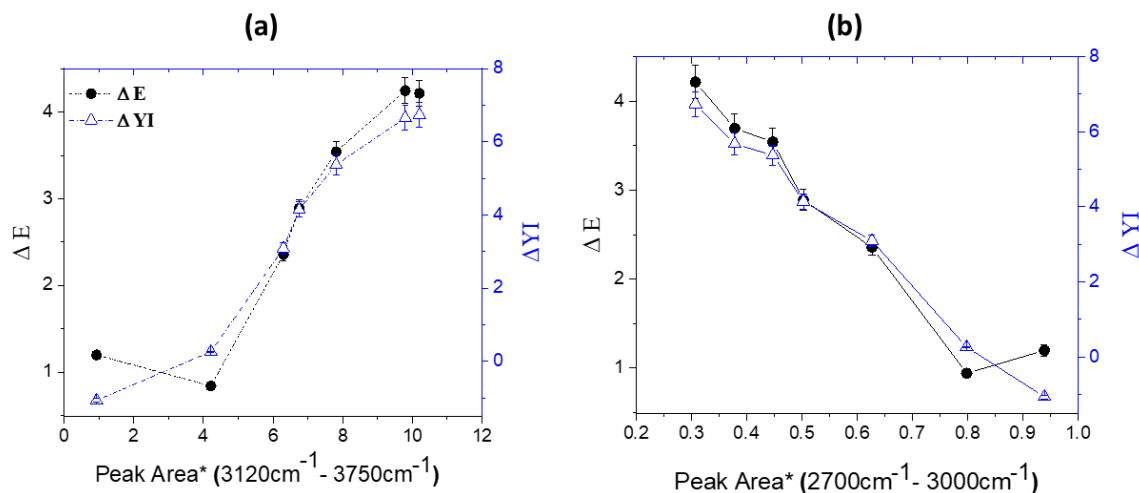
Fig. 9. Changes in color appearance at SPHERE (55 °C, 75 % RH) exposure conditions vs. changes in IR peak area in (a) hydroxyl region (3120 cm^{-1} to 3750 cm^{-1} ) and (b) hydrocarbon region (2700 cm^{-1} to 3000 cm^{-1} ). Peak areas are normalized by the peak area at 0 MJ/m^2 . Data points indicate the mean and the error bars (one standard deviation, 5 replicates).
