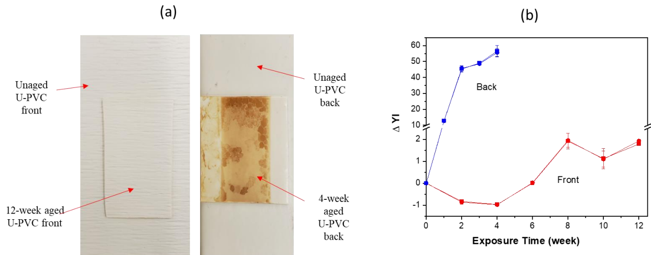
Fig. 7. (a) Photos of U-PVC surfaces (front and back) before and after QUV aging; (b) corresponding yellowness index ( \Delta YI ) as a function of exposure duration in QUV. Data points indicate the mean, and the error bars the standard deviation (5 replicates).
