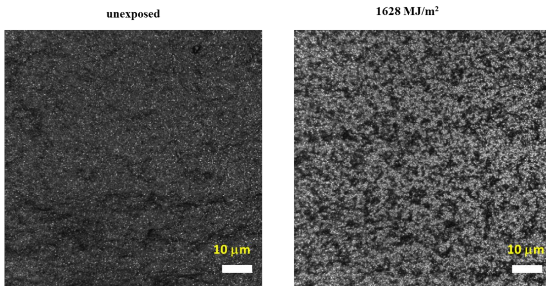
Fig. 10. LSCM images of front U-PVC before and after exposure in SPHERE ( 1628 \text{ MJ/m}^2 , 55 °C, 75 % RH)
