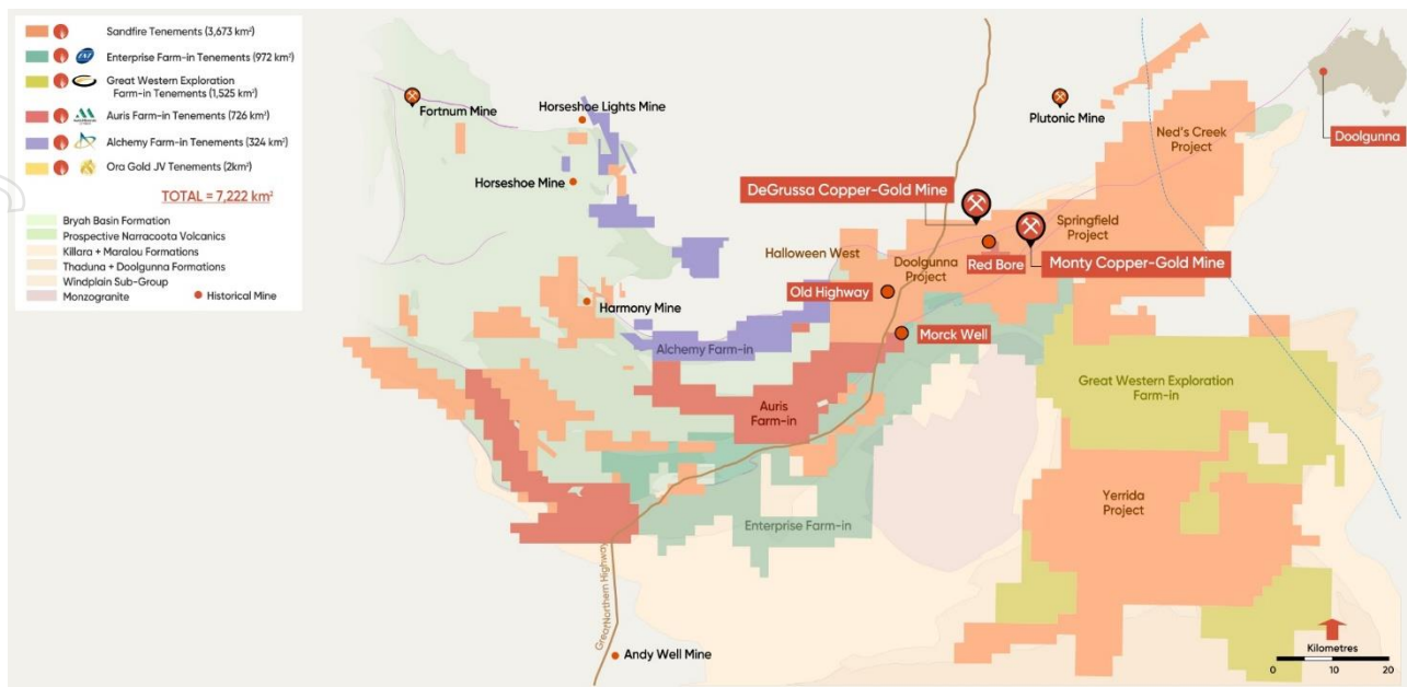
Figure 1 – DeGrussa and Monty Copper-Gold Mine Location.
