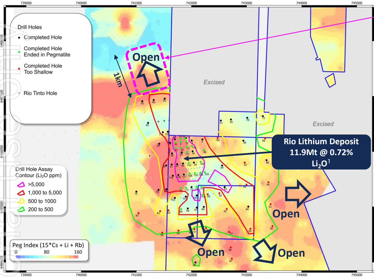
Lithium Contours from Drilling over Image of Soil Geochemistry
