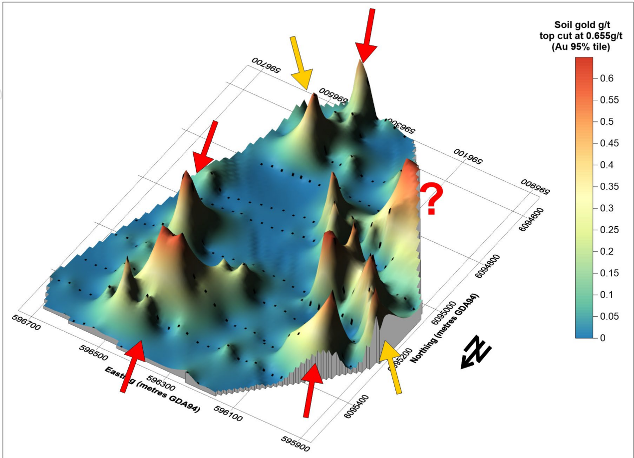
Figure 2 – The combined soil sampling program results showing linear trends with very elevated gold in the soil. All soil gold values above 0.655 g/t Au were reduced to that value for this image. The orientation of the elevated mineralisation on the southwest side is unknown.
