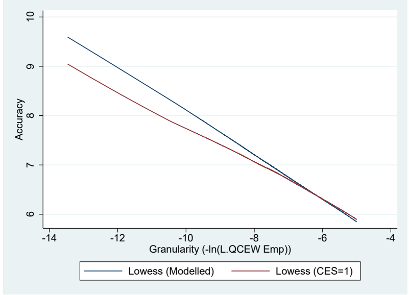
Figure 7: Production Frontier for County-level Estimates: Fitted Lowess Values of Accuracy and Granularity
