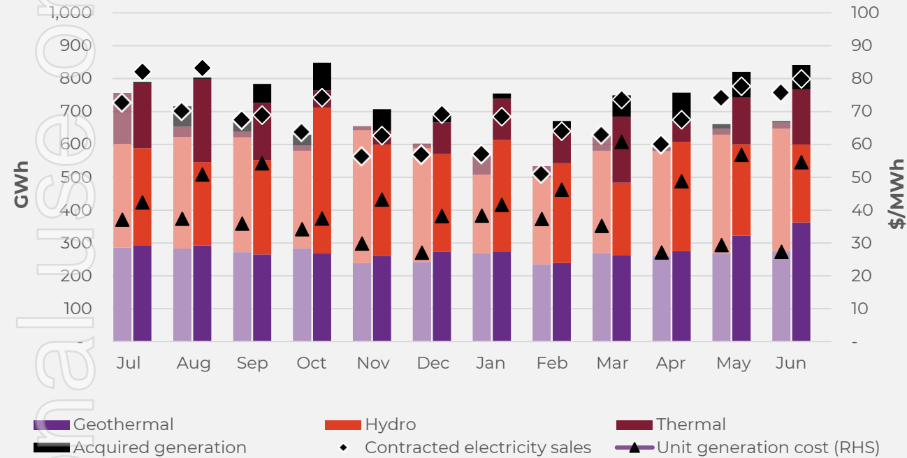
Generation mix, gross sales position and unit generation cost (FY23 and 24 respectively)
