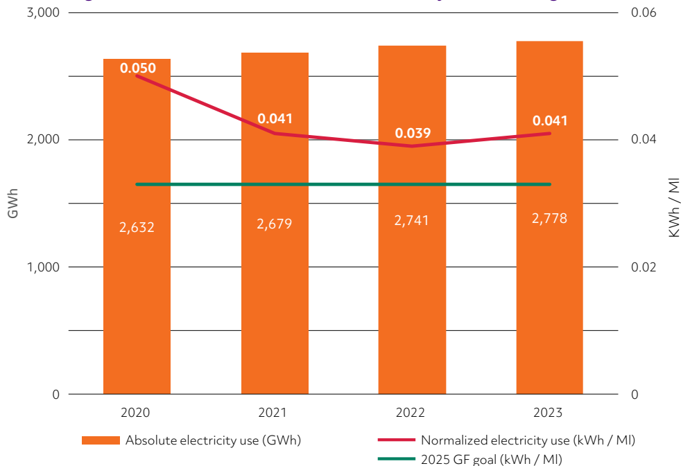
Figure 10. Absolute and normalized electricity use — through 2023
