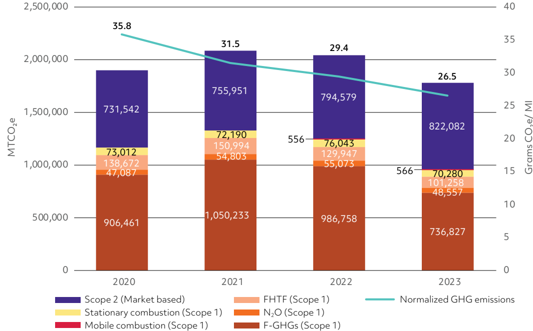
Figure 8. Absolute and normalized direct (Scope 1) and indirect (Scope 2) GHG emissions — through 2023 21,22
