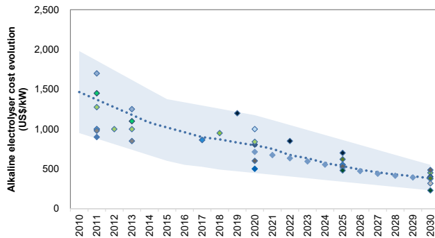
Exhibit 63: There exist a wide range of estimates for both the historical and future trajectory of electrolyzer system costs.. Alkaline electrolyzer system cost (US$/kW)
