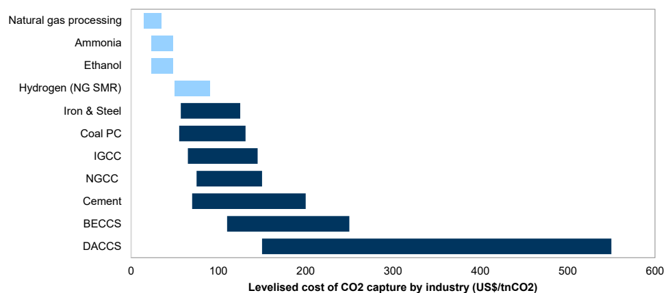
Exhibit 181: The levelized cost of carbon capture depends on the concentration of CO 2 in the capture stream. Lower concentration typically requires more energy and cost in capturing. Levelized cost of CO 2 capture by industry
