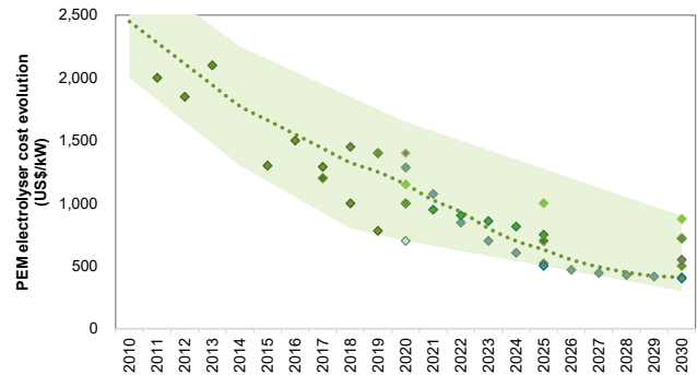
Exhibit 64: ..with PEM electrolyzer systems costs currently screening higher than the competing alkaline technology costs owing to PEM's more recent technological development PEM electrolyzer cost evolution (US$/kW)
