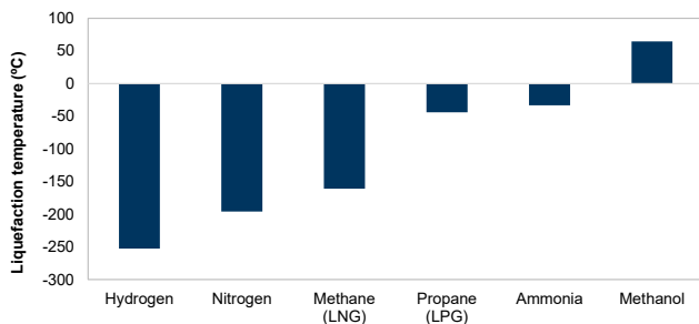
Exhibit 91: The very low liquefaction point of hydrogen makes liquefaction more energy intense/costly compared to natural gas..
