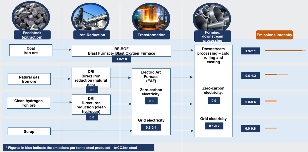
Exhibit 143: Schematic summary of possible steel manufacturing routes and associated emissions intensity (tnCO2eq/tn steel)
