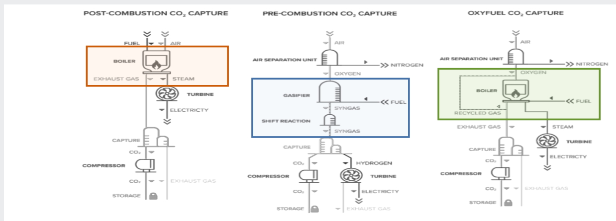
Exhibit 180: There exist different CO 2 capture processes for use in power generation and industrial plants CCS
