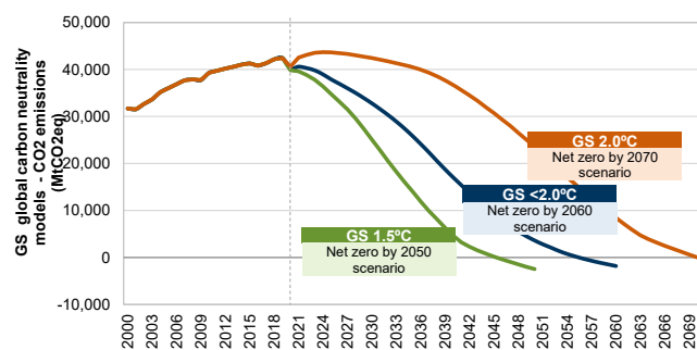
Exhibit 44: We leverage our three global GS net zero carbon models, each consistent with a specific carbon budget and resulting temperature rise..
