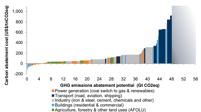
Exhibit 29: ...leveraging our global Carbonomics cost curve of de-carbonization 2021 Carbonomics carbon abatement cost curve for anthropogenic GHG emissions, based on current technologies and current costs
