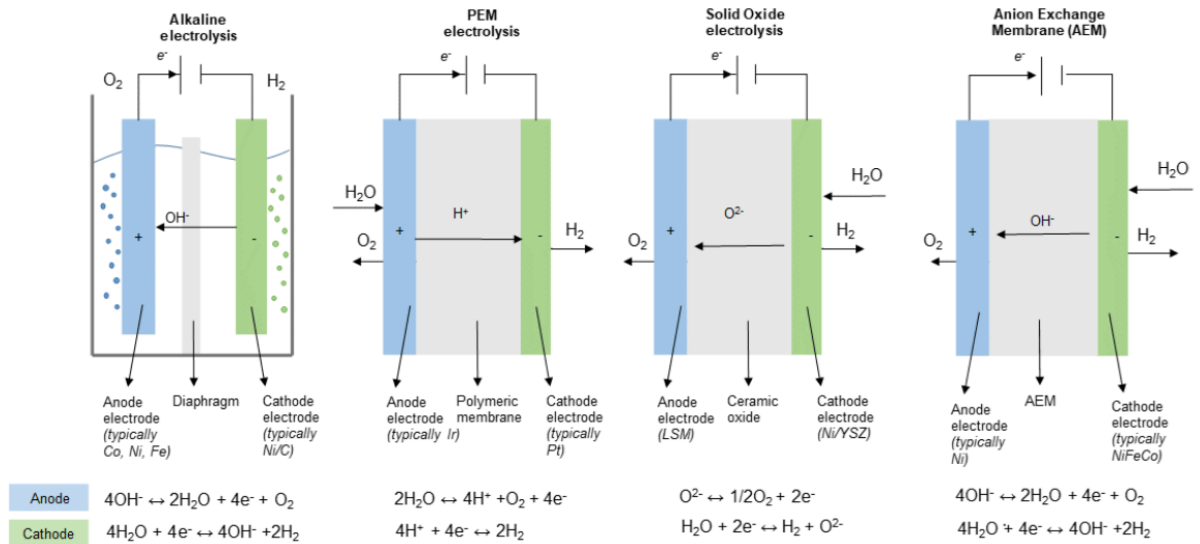
Exhibit 60: Simplified schematic of the three currently commercialized electrolysis technologies for the production of 'green' hydrogen
