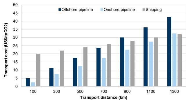
Exhibit 183: ..and for smaller distances, as shipping becomes more economically attractive for distances >1000km Transport cost of CO 2 (US$/tnCO 2 )
