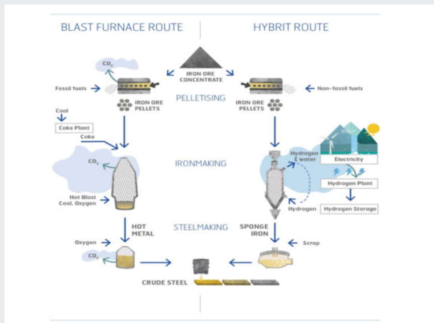
Exhibit 144: HYBRIT process route schematic diagram
