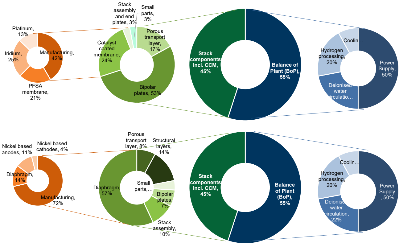
Exhibit 65: Cost breakdown for a typical 1 MW PEM electrolyzer (top) and alkaline electrolyzer (bottom)
