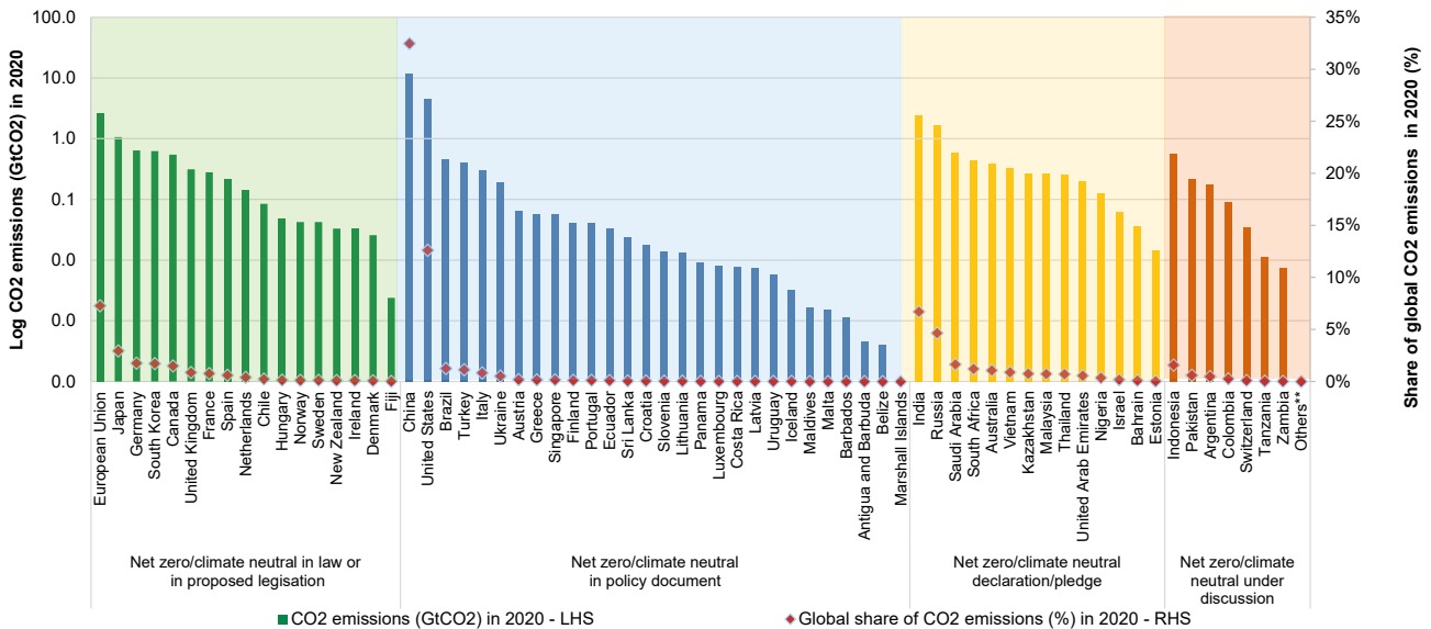
Exhibit 30: The rapidly rising number of national net zero/climate neutral pledges (including those in law, legislation and policy documents) worldwide by YE2021 covered c.83% of the global CO2 emissions, of which around half have a timeline for net zero by 2050 or sooner (the key exception being China)
