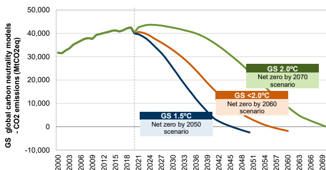
Exhibit 28: We have constructed three global carbon neutrality models: one consistent with 1.5°C of global warming, one consistent with well below 2.0° and one consistent with 2.0°.. GS global net zero models, CO2 emissions (incl. AFOLU)
