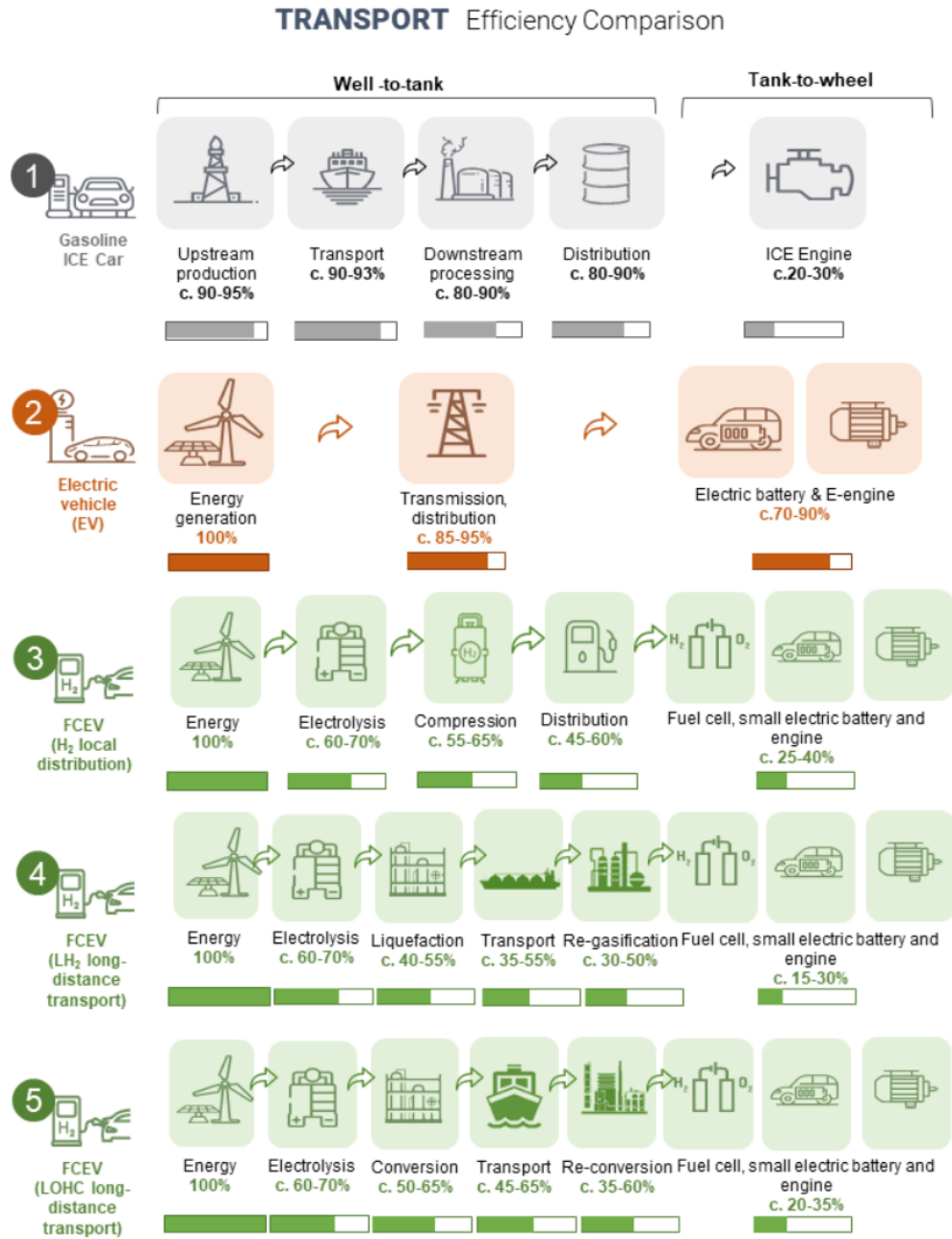
Exhibit 157: Hydrogen has low efficiency, on a comparative basis, with electric vehicles being twice as efficient on a well-to-wheel/power-to-wheel basis
