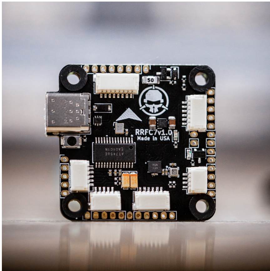
Rotor Riot Brave F7 Flight Controller
