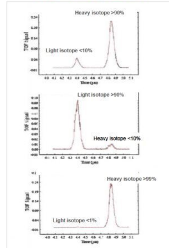
Laser Enrichment of Lithium 6
