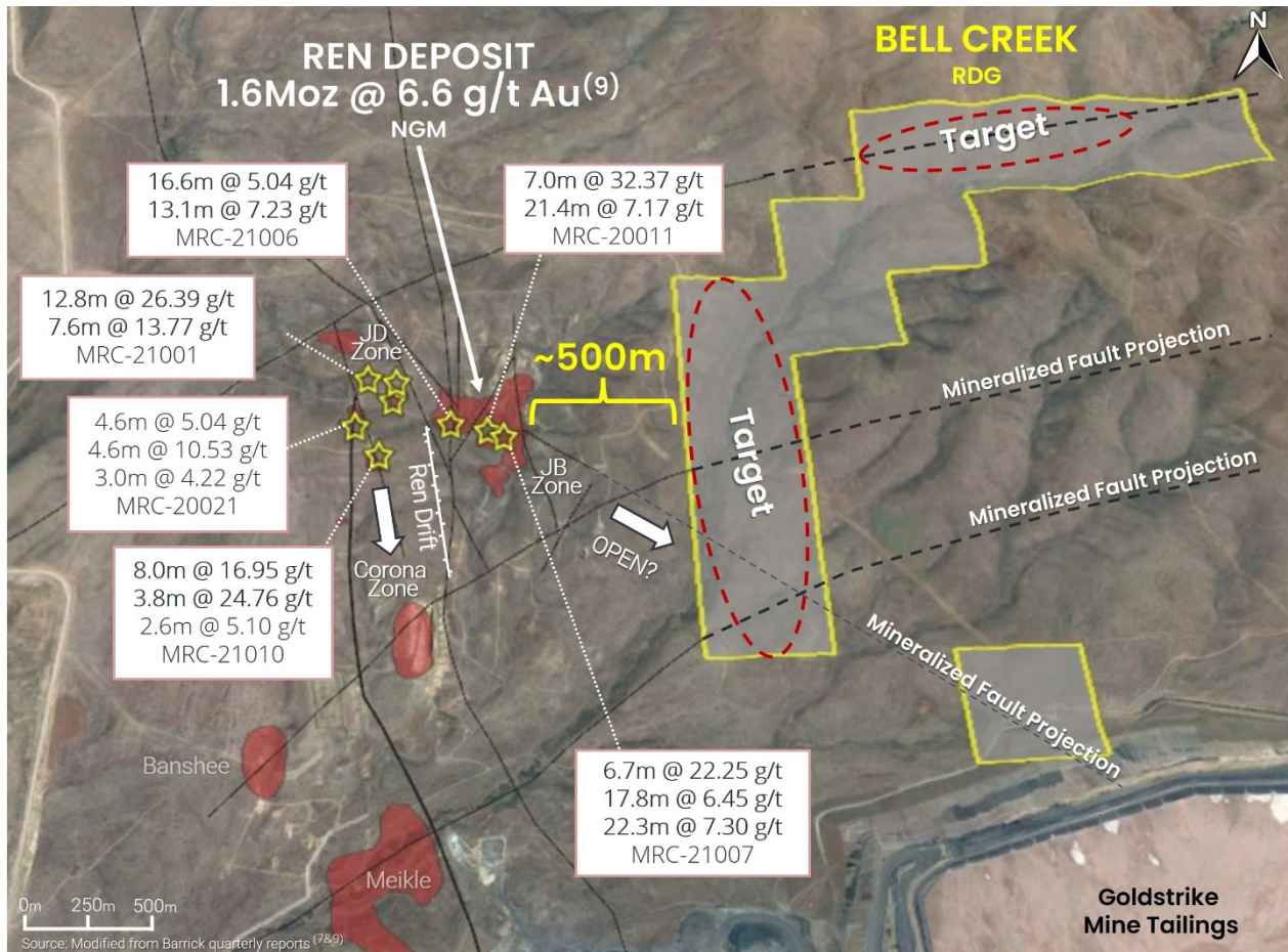
Figure 16: Zoomed in map of the Ren Deposit resource and Bell Creek project with multiple fault structures interpreted as projecting onto the Bell Creek property.
