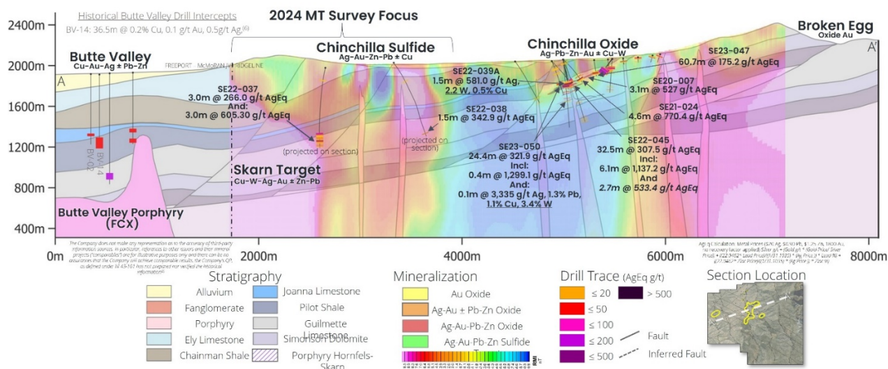
Figure 6: Long Section A-A' showing high-grade drill intercepts at both the Chinchilla Oxide and Chinchilla Sulfide targets overlying the Company's 2023 3D magnetic inversion. High-grade mineralization is located at the intersection of NW and NE fault zones (ie: chimney horizons) intruded by quartz-feldspar porphyry dikes.
