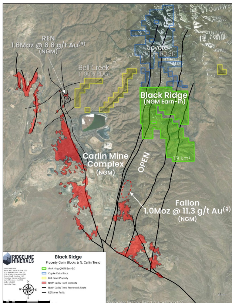
Figure 15: Plan view map of the North Carlin Trend showing location of the Bell Creek project in relation to Ridgeline's Black Ridge earn-in agreement with NGM and the NGM owned Ren deposit, which released a maiden resource of 1.6 Moz grading 6.6 g/t Au in Q1 2022.
