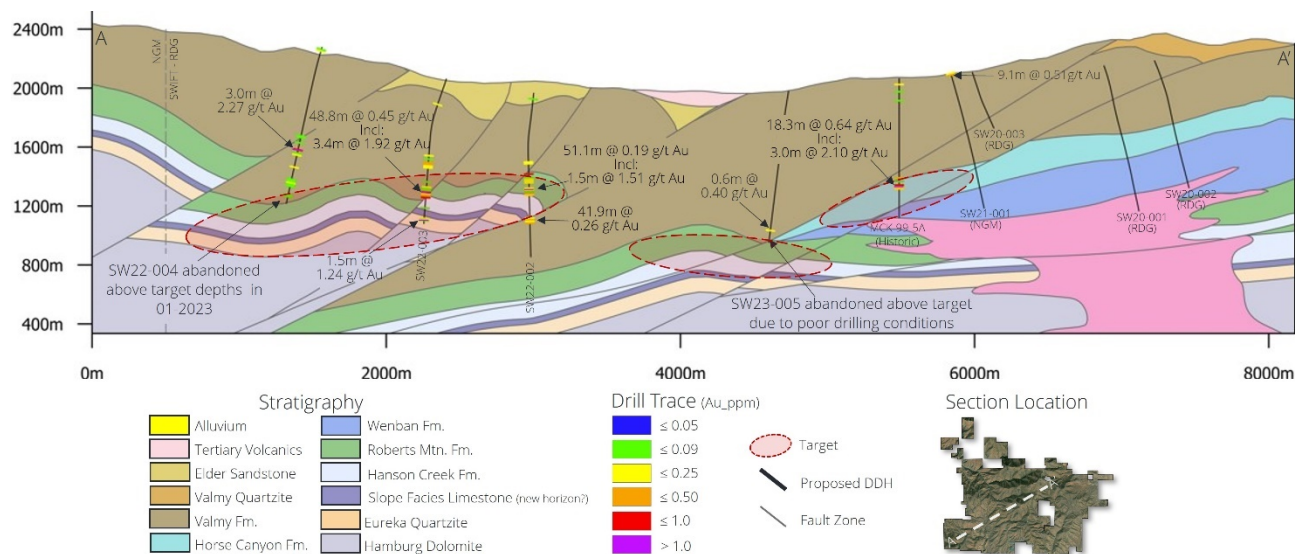
Figure 9: Long Section showing the widespread “framework” drillholes completed by NGM between Q4 2021 and Q4 2023.
