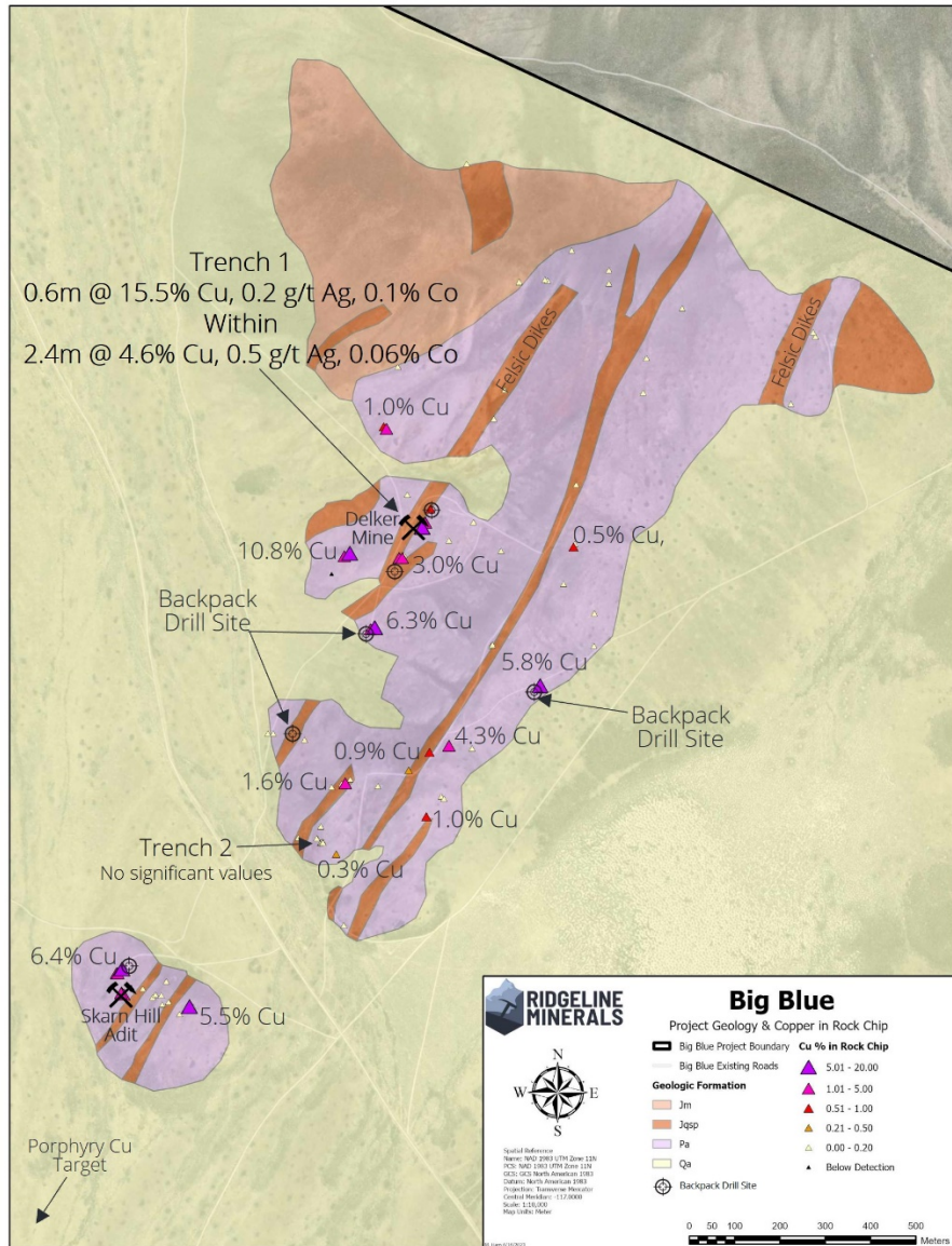
Figure 14: Plan view map of the Delker Mine area showing high-grade trenches and rock chips (Cu%). Mineralization directly associated with NE trending felsic dike swarm
