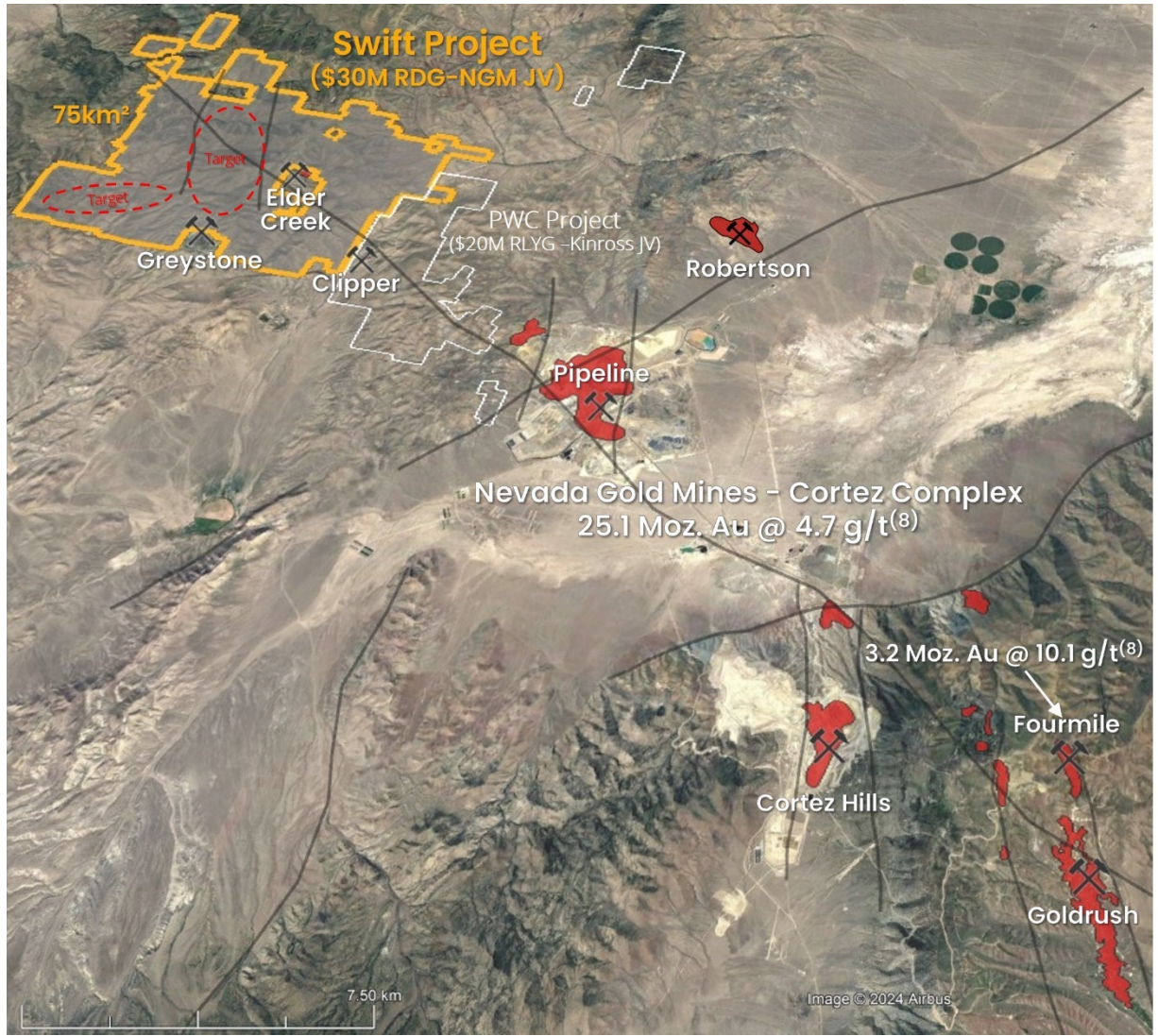
Figure 7: Modified Google Earth image showing location of Swift Project in relation to Cortez District gold mines along the Battle Mountain-Eureka Trend.
