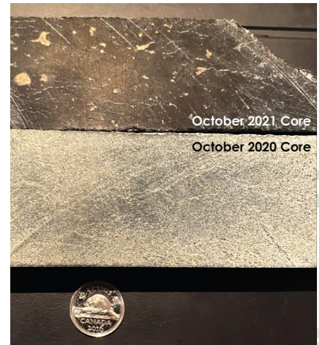
Drill Core Oct 2021 vs Oct 2020 Spontaneous Carbonation (white minerals)
