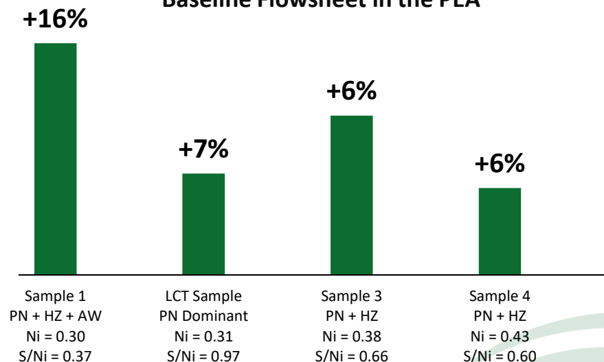
Improved Ni Flotation Recovery compared to the Baseline Flowsheet in the PEA
