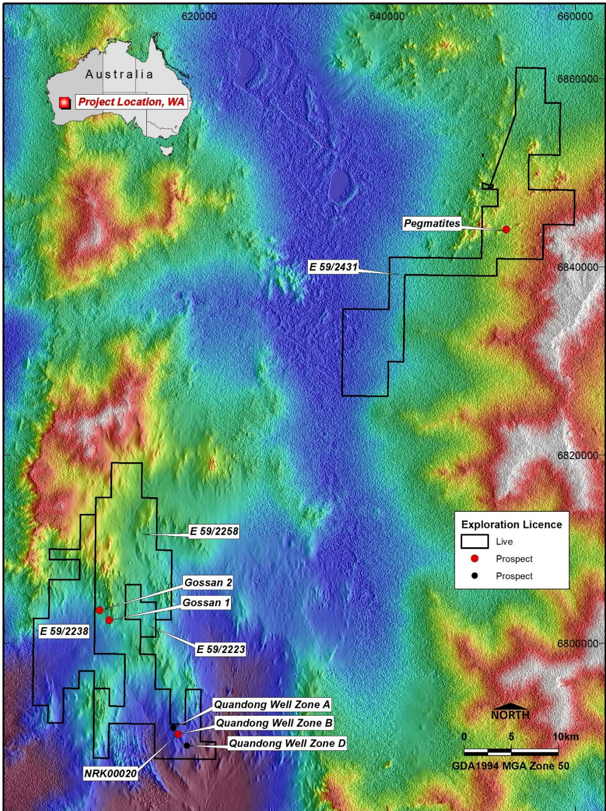
Figure 9. Digital elevation image from the new broader aeromagnetic data compilation over the NIC
