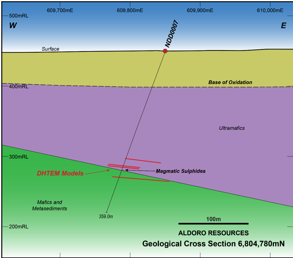
Figure 6. Cross-section of NDD0007 at 6804780m north (MGA50)
