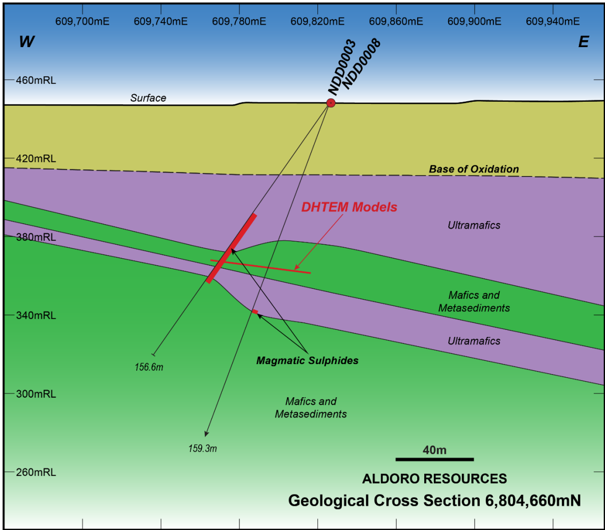
Figure 4. Cross-section of NDD0003 and NDD0008 at 6804660m north (MGA50). Note the possible identification of a "choke point" or structural trap at NDD0008, where the thicker accumulation of magmatic sulphide is occurring.
