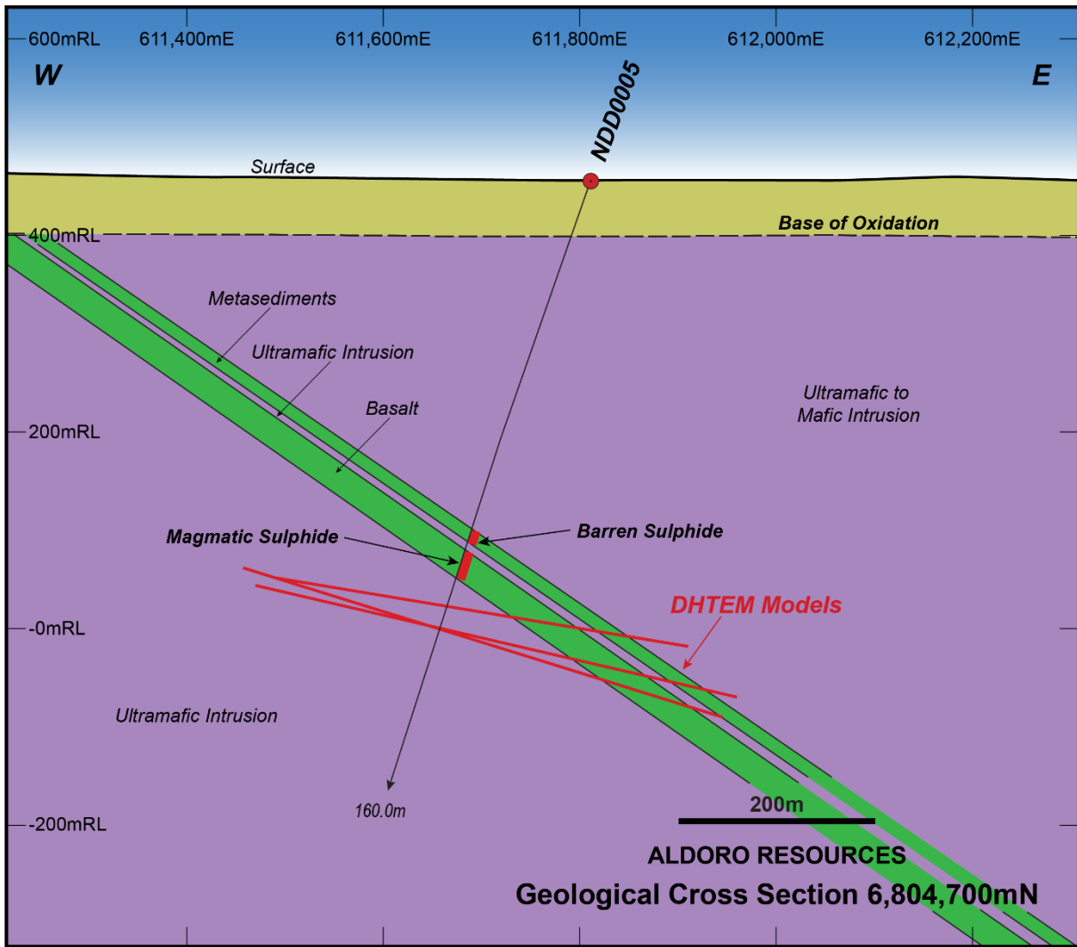
Figure 7. Cross-section of NDD0005 at 6806700m north (MGA50), the first hole into the VC3 target.
