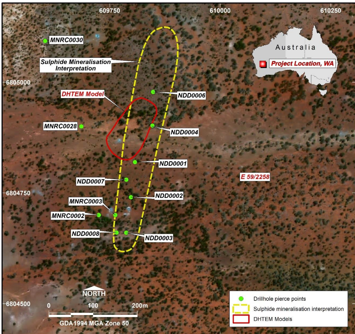
Figure 2. Plan projection showing completed drillhole pierce points of the VC1 target and an evolving interpretation of the magmatic sulphide footprint. DHTEM surveying generated a revised off-hole target shown in red.
