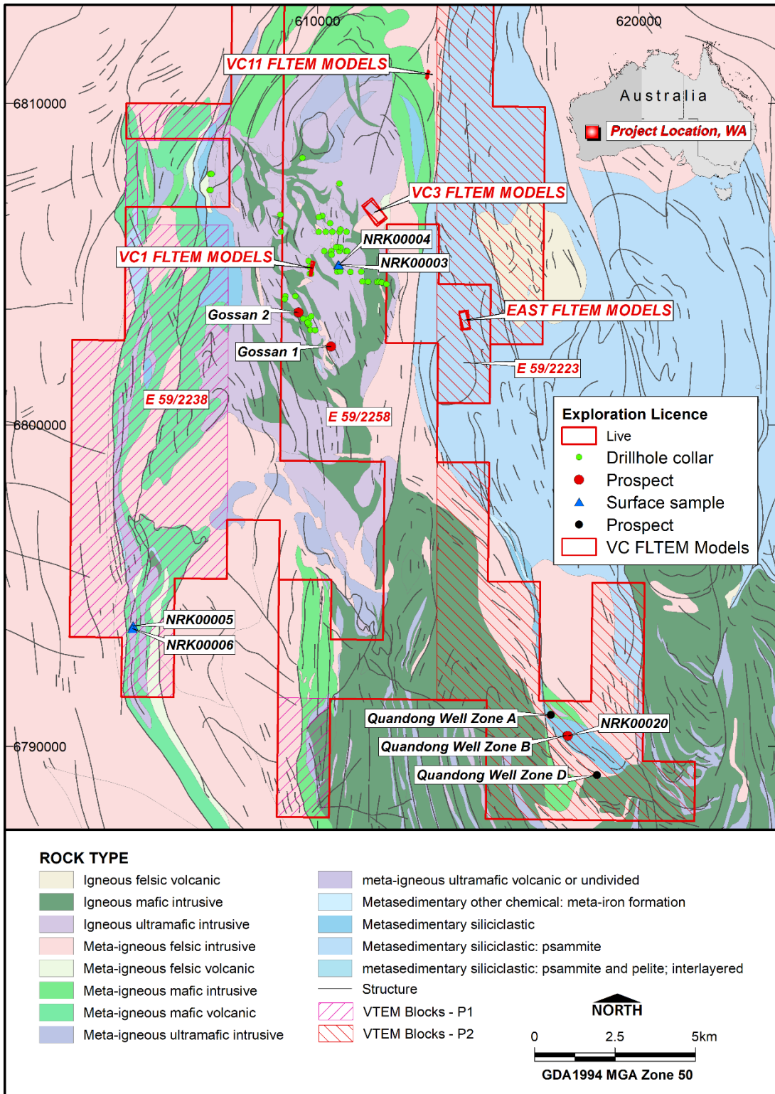
Figure 8. Geological map of the NIC, showing the location of all relevant targets and the proposed VTEM extension surveys.
