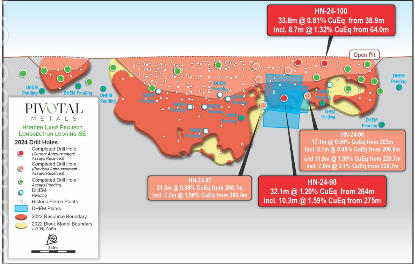
Figure 2 is a longitudinal section showing the spatial distribution of historical and new drill hole pierce points, and DHEM plates associated with the reported survey holes.
