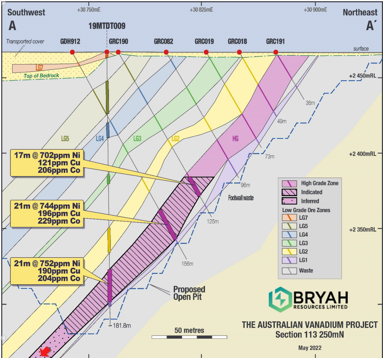
Figure 3 – Cross Section at 113 250 mN showing geology model and location of the base metals Mineral Resource categories
