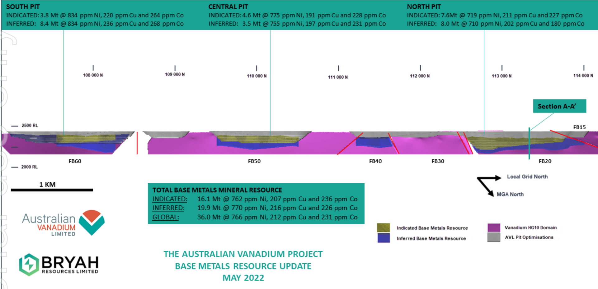
Figure 2 – Base Metals Mineral Resource Category Long Section – Local Grid, looking West.
