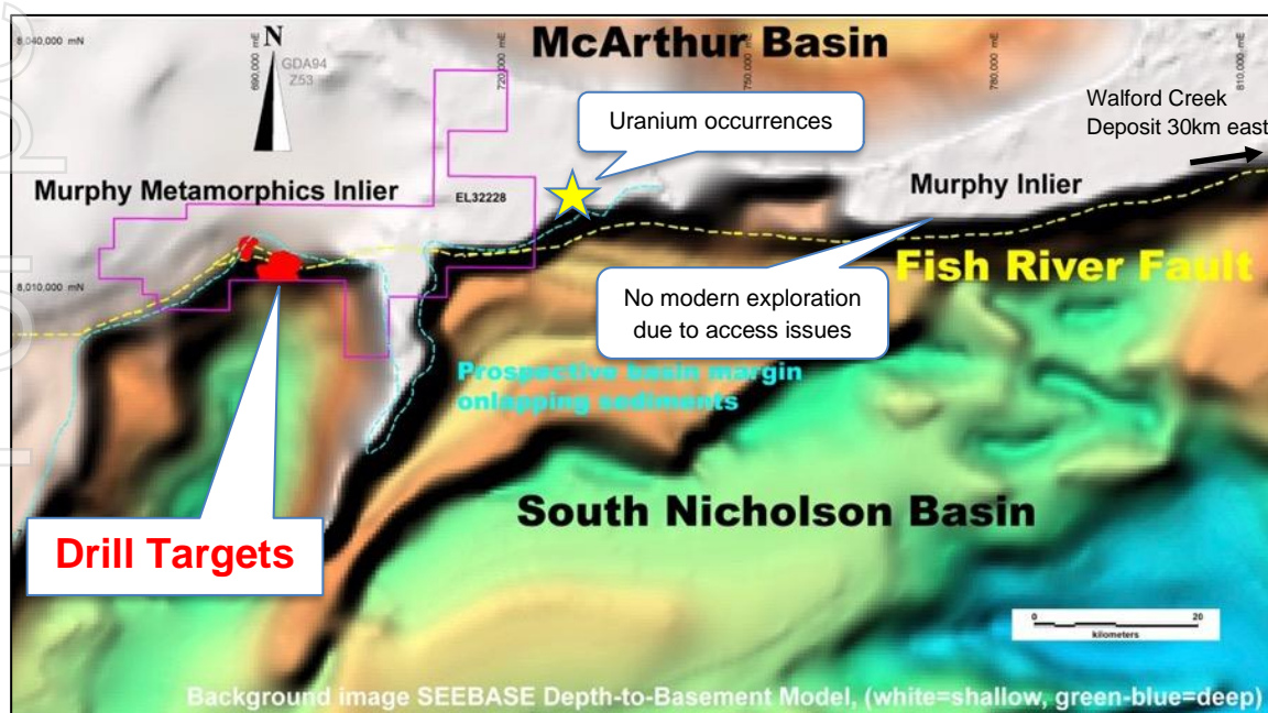
Figure 3 Drill targets and regional setting, with interpreted extension of the Fish River Fault from QLD to the project
