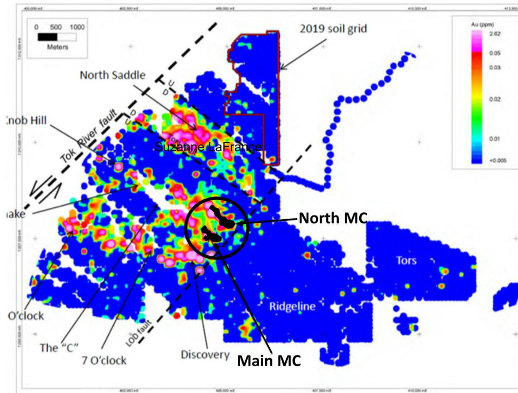
Chief Danny Area: Gold in Soils (thru 2019)
