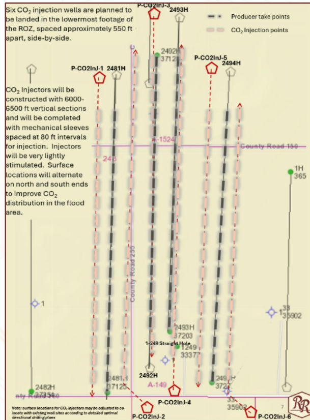
Top View
