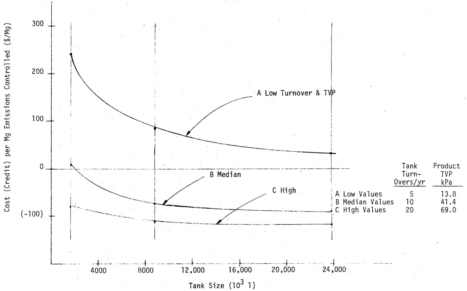
Figure 4-2. Cost Effectiveness of Controlling Emissions From Existing Fixed Roof Crude Oil Tanks
