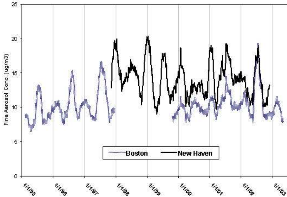
Figure 3-7. Moving 60-day average of fine aerosol mass concentrations based on long-term data from two northeastern cities
