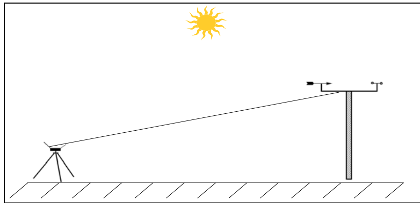
Figure 2.13 Side View of the Placement of a Compass or Transit for Measuring the Crossarm Direction
