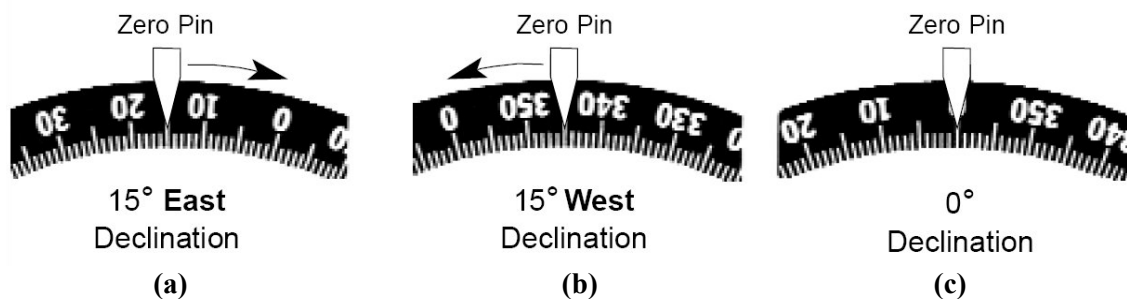
Figure 2.12 Adjusting for (a) East and (b) West Declinations; (c) No Adjustment for Magnetic Declination of 0^\circ
