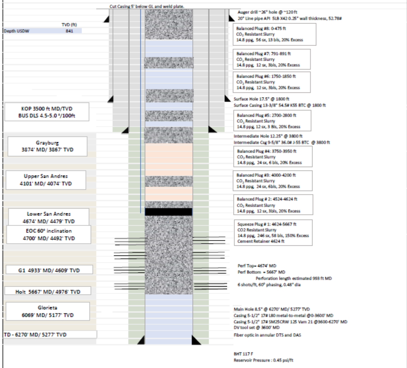
Figure 1—BRP CCS1 well plugging schematic
