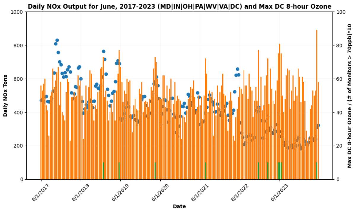
Figure 6: Daily aggregate NO x , maximum DC ozone, and monitors exceeding 70 ppb in May 2017-2023.
