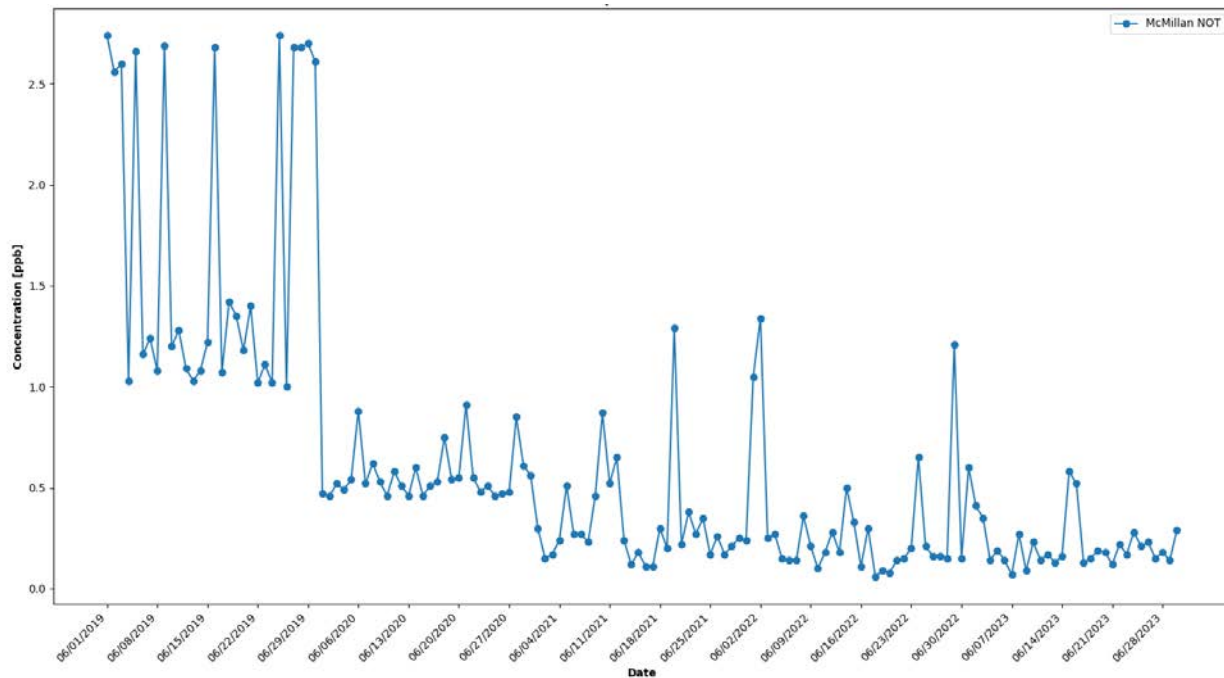
Figure 35: NOT concentrations from McMillan monitor for days in June from 2019 to 2023.
