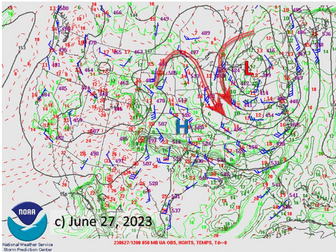
Figure 14: Figure 13, as in Figure 11, but for a) June 25, b) June 26, and c) June 27.
