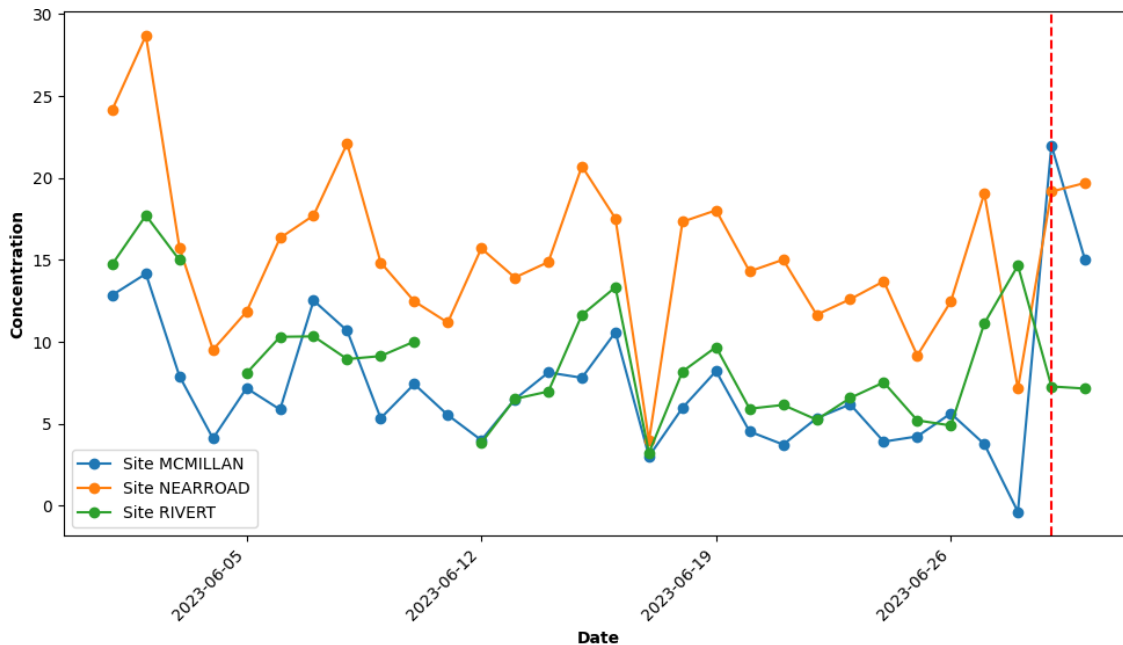
Figure 33: As in Figure 28, except for daily average nitrogen dioxide (NO 2 ) from available District monitors in June 2023.
