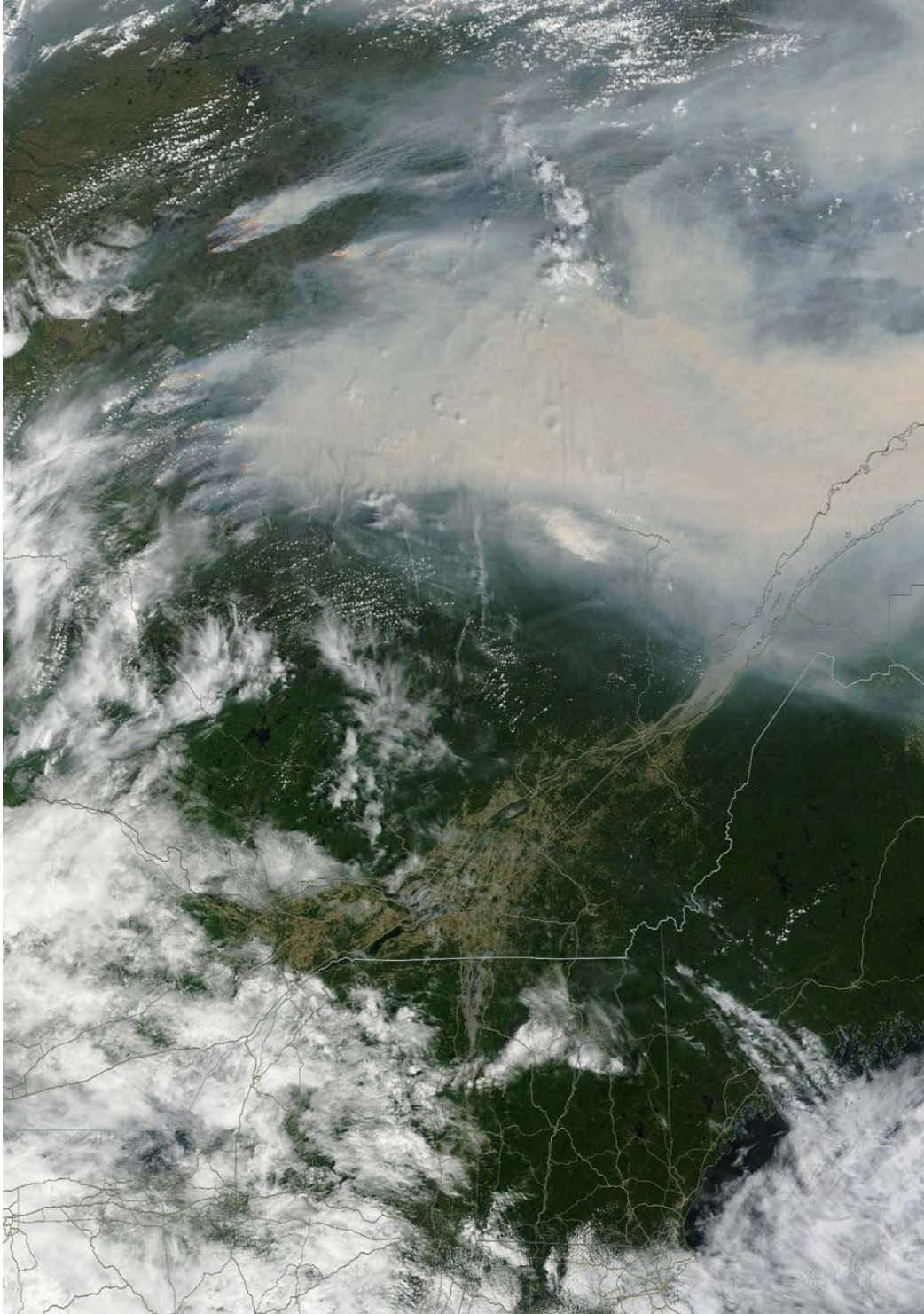
Figure 10: June 23, 2023, Terra/MODIS Corrected Reflectance with overlaid Terra/MODIS Fires and Thermal Anomalies
