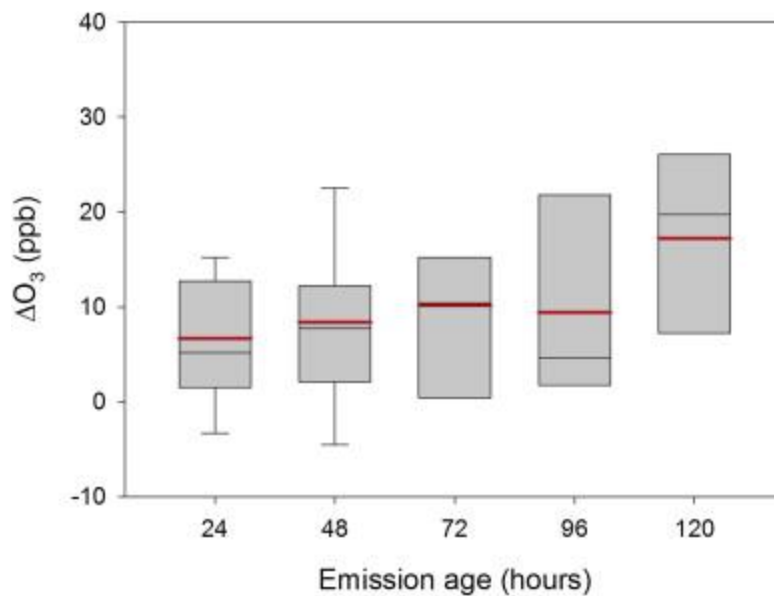
Figure 11: Ozone enhancement with smoke plume age. (from Putero et al. (2014), Figure 7)
