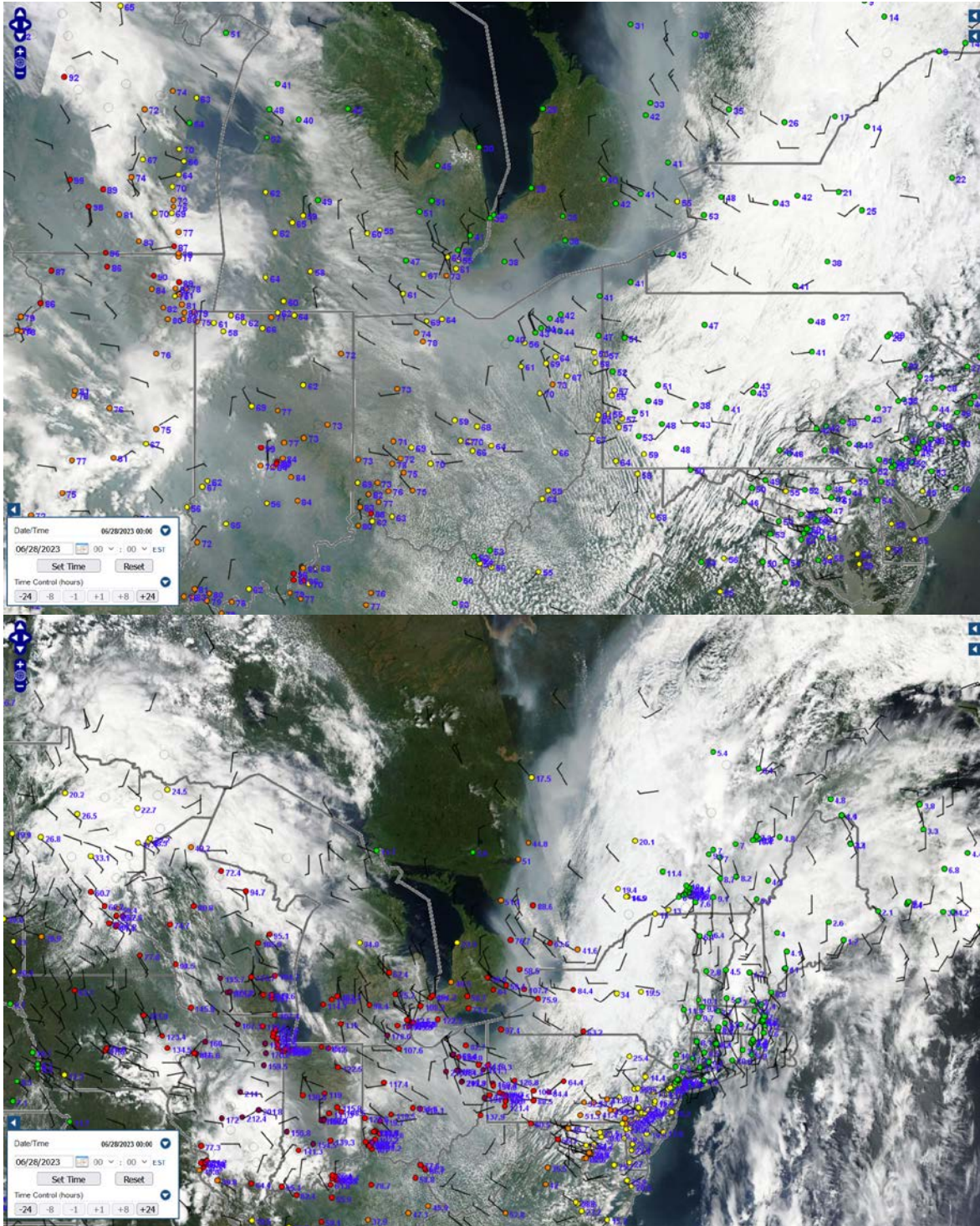
Figure 18: June 21-28 maximum daily 8-hour average ozone and daily average PM2.5 concentrations across eastern CONUS.
