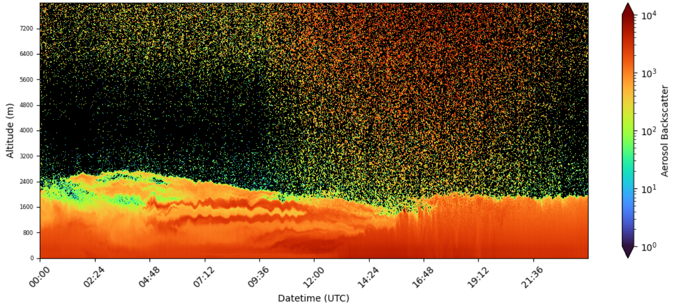
Figure 25: Ceilometer backscatter (colors) from a) The McMillan Reservoir site on June 29, 2023.
