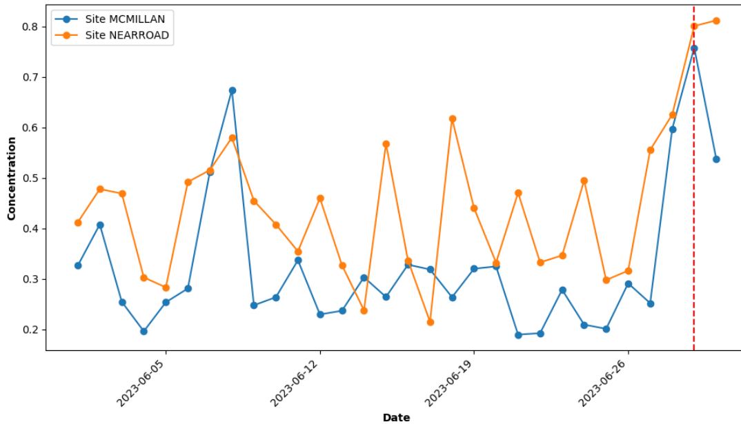
Figure 30: Daily Carbon Monoxide (CO) at available sites in the District on June 29 th is highlighted by the red vertical lines.
