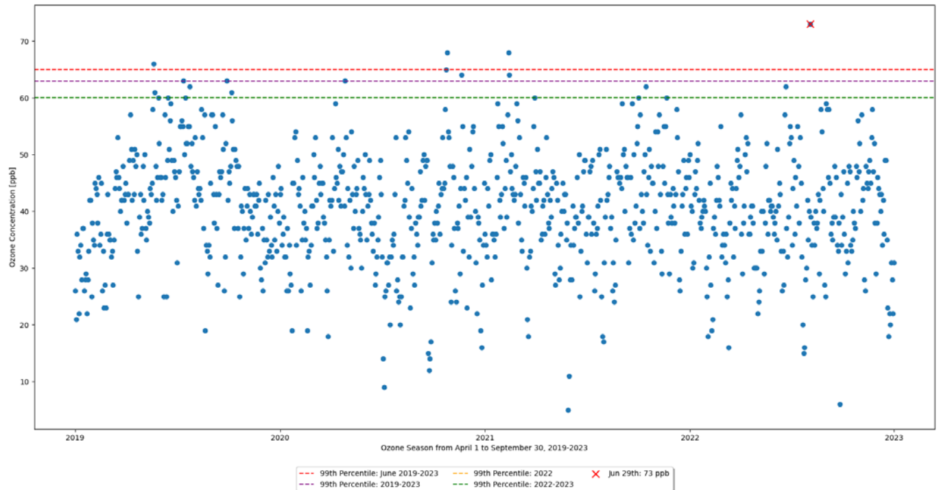
Figure 21: Scatterplot of Maximum Daily 8-hour Average Ozone (MD8AO) concentrations at River Terrace (blue dots), April 1 – September 30, 2019-2023.
