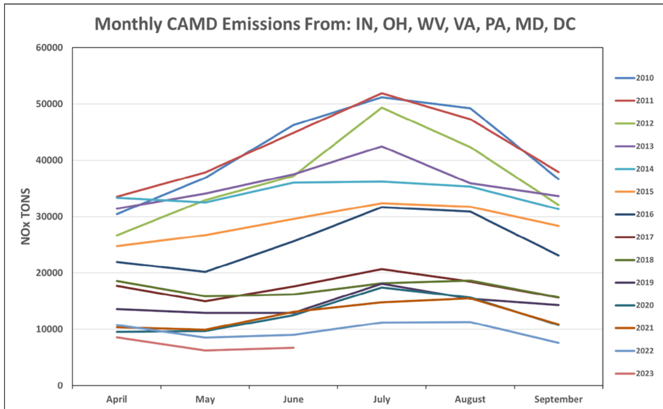
Figure 5: Monthly NO x -aggregated from the group of upwind states, including the District by Month of ozone season.
