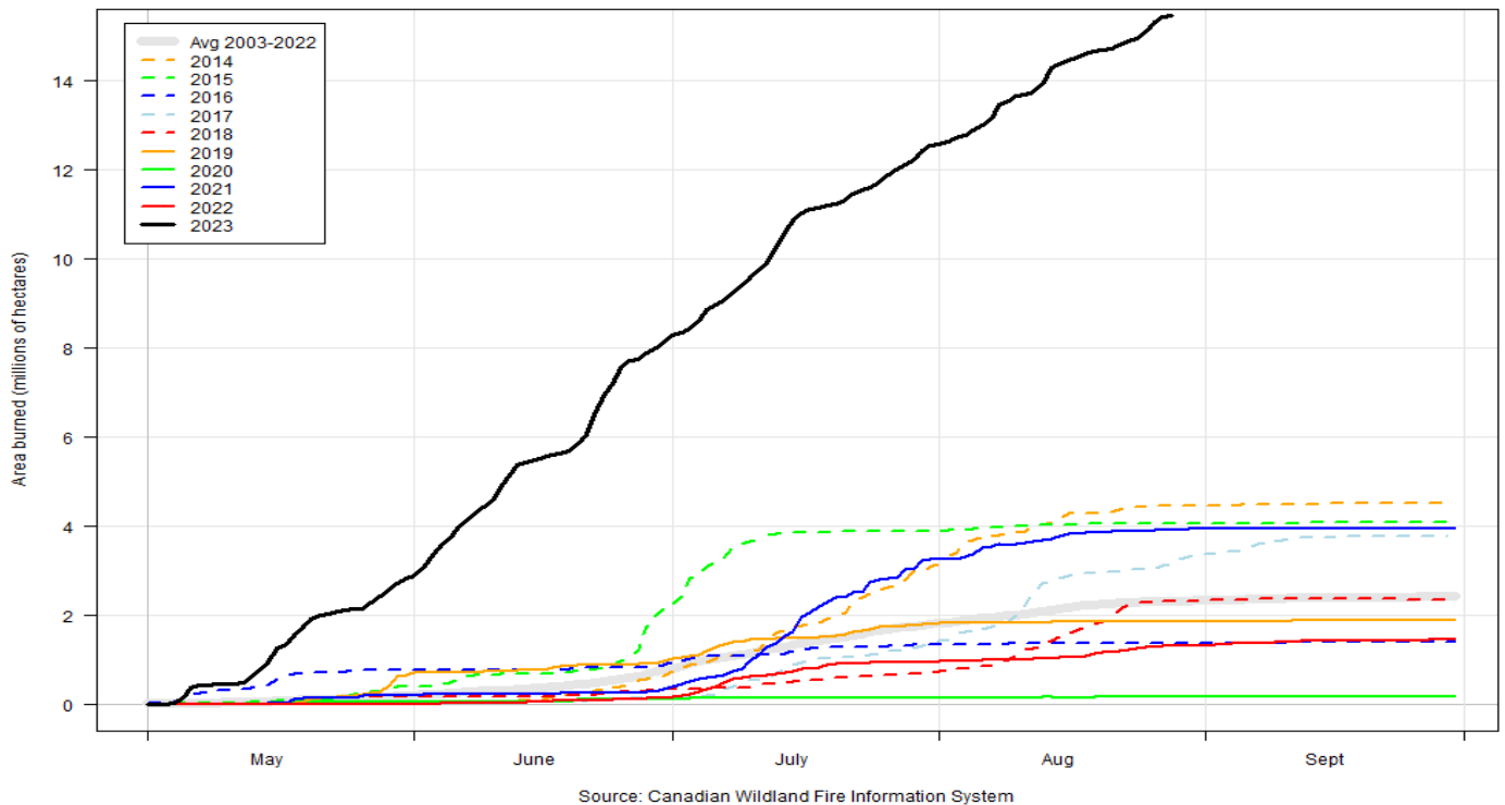
Figure 8: Cumulative hectares burned reported by the Canadian Wildland Fire Information System (CWFIS) by day over the last ten years. The burn area is estimated by satellite.
