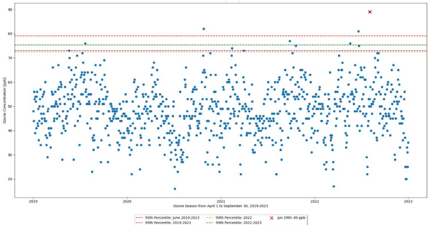
Figure 20: Scatterplot of Maximum Daily 8-hour Average Ozone (MD8AO) concentrations at McMillan (blue dots), April 1 – September 30, 2019-2023.
