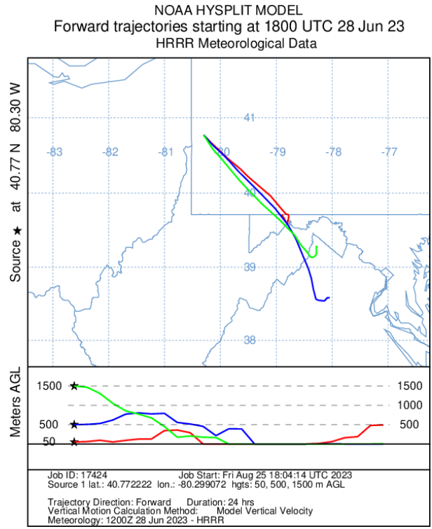
Figure 26: HYSPLIT 24-hour forward trajectories based on HRRR meteorology on June 28, 2023, at 2 pm (1800 UTC) from an area of dense smoke observed over western Pennsylvania.
