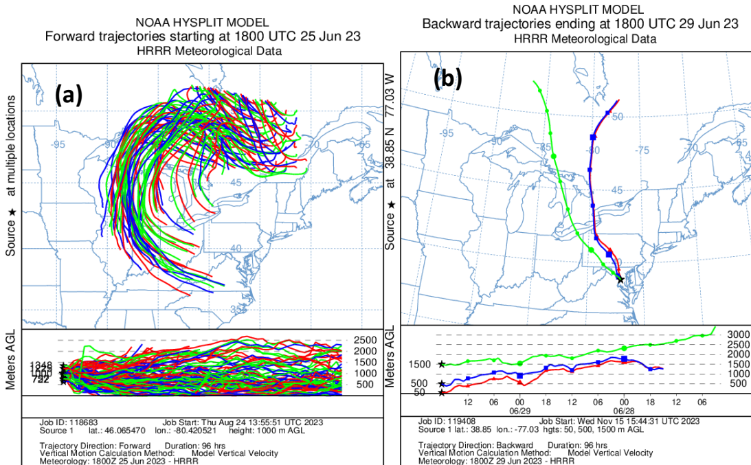
Figure 22: Forward and Backward Transport Trajectories (a) A Matrix of 96-hour (4-day) High Resolution Rapid Refresh (HRRR) forward trajectories with starting points centered around the location of the maximum smoke concentrations in Quebec on June 25, 2023.
