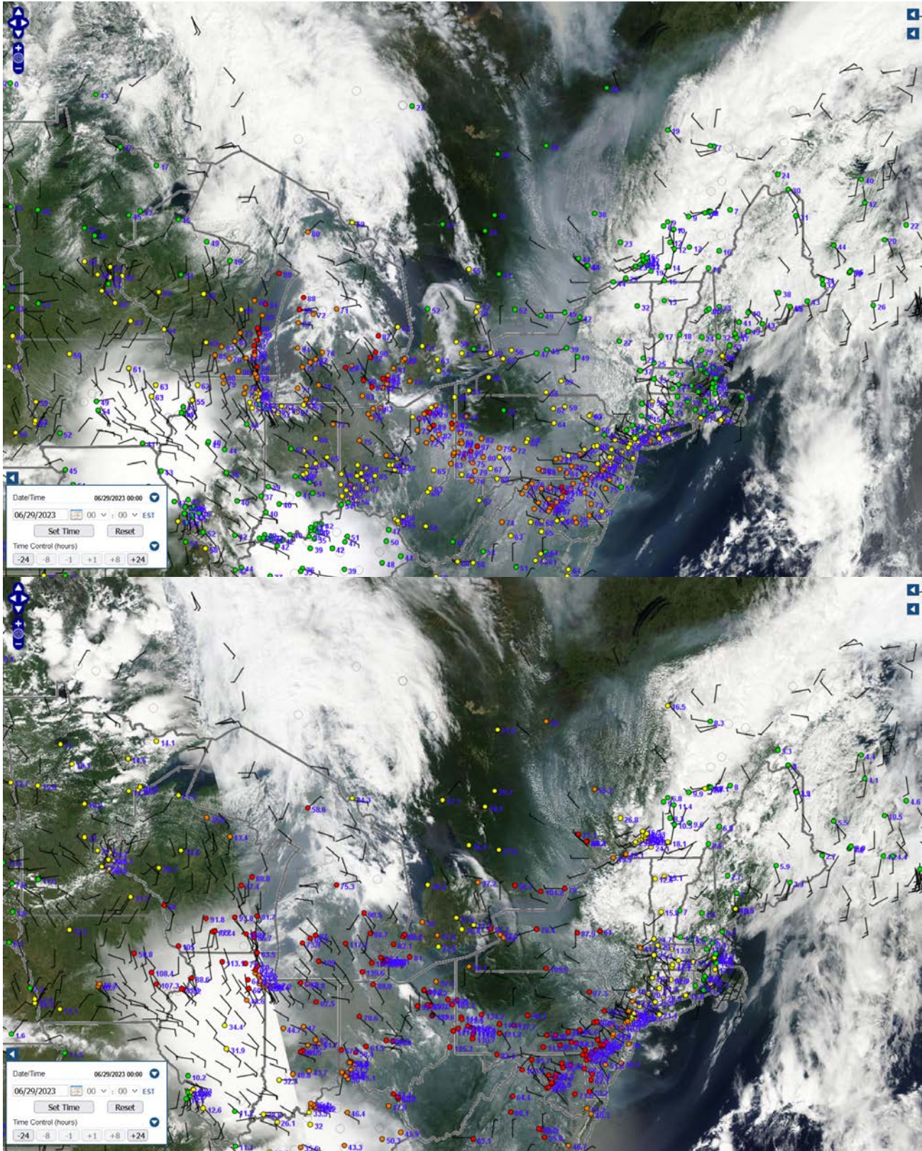
Figure 19: As in Figure 17, but for June 29 th
