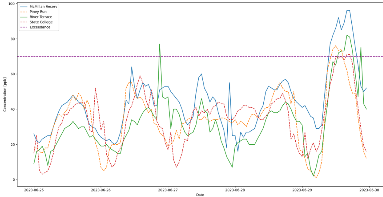
Figure 31: Comparison of hourly ozone concentrations from both urban District monitors vs rural monitors Piney Run (Maryland) and State College (Pennsylvania) from June 25th -June 29th.
