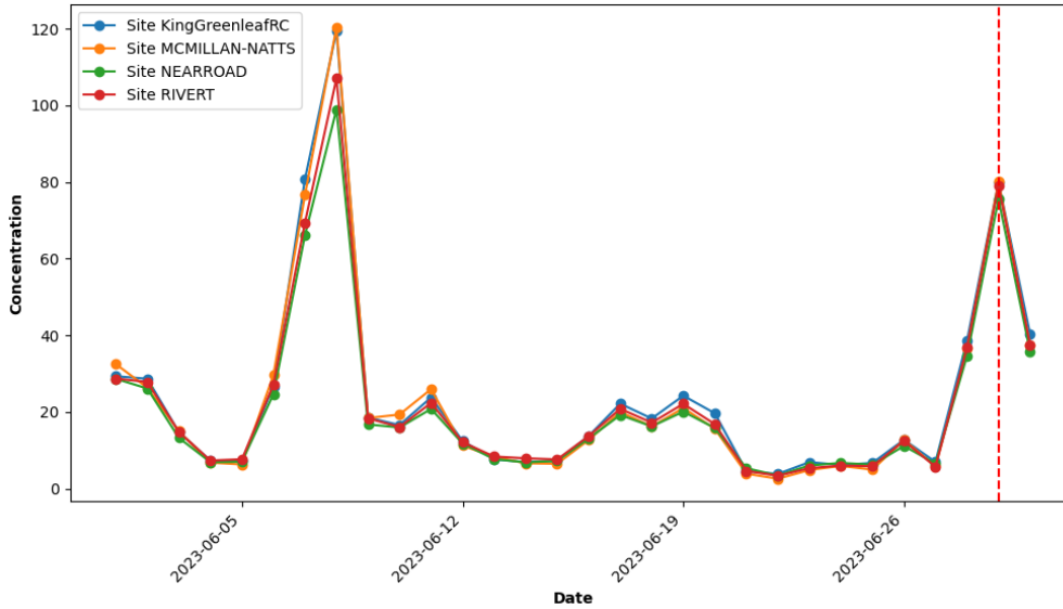
Figure 29: Daily averaged fine particle (PM 2.5 ) concentrations for all sites available in the District for the month of June 2023. June 29 th is highlighted by the red vertical line.
