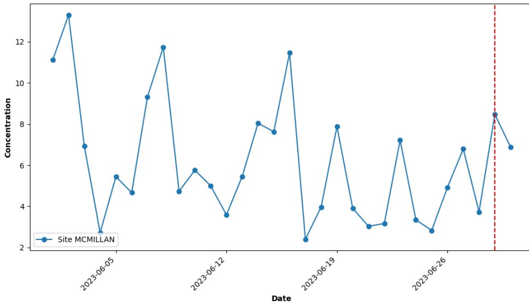
Figure 34: Daily oxides of Nitrogen concentrations at the District's McMillan site for the month of June.
