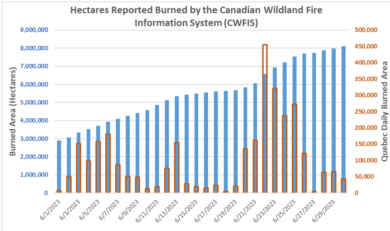
Figure 28: Hectares burned reported by Canadian Wildland Fire Information System (CWFIS).
