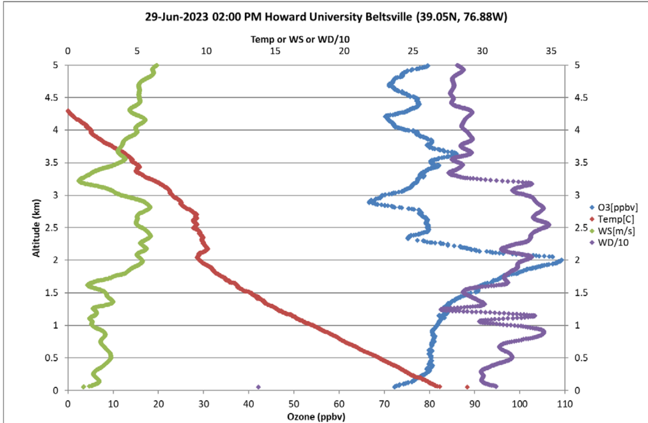
Figure 27: Same as figure 22 but for June 29, 2:00pm (1800 UTC)
