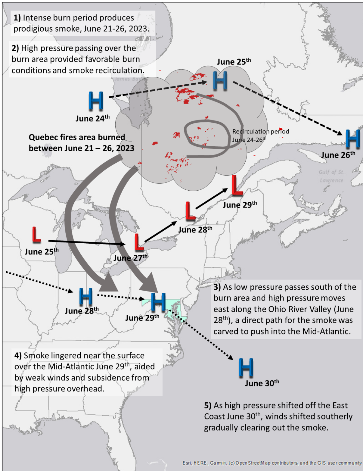
Figure 12: A simplified, illustrated conceptual model of the June 29, 2023, wildfire-influenced ozone event.
