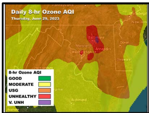
Figure 1: AQI maps from June 29, 2023.
