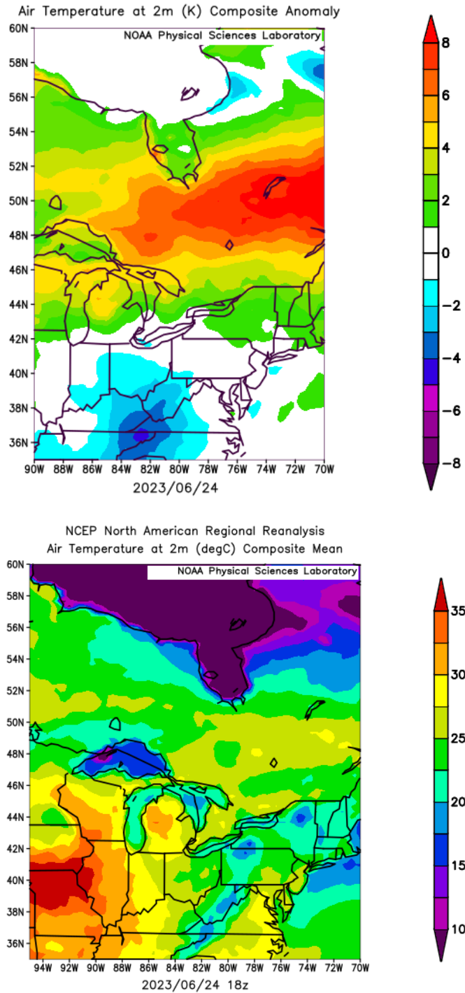
Figure 17: 2 pm (EDT) temperature on June 24, 2023, from the North American Regional Reanalysis (NARR).
