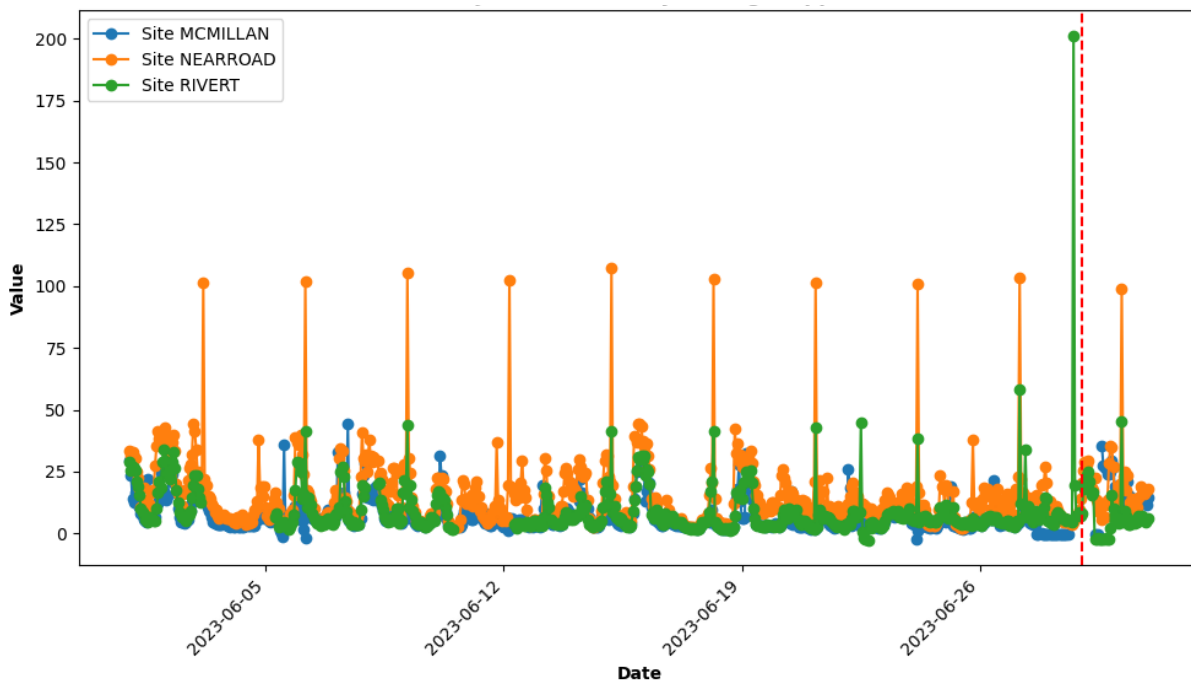
Figure 32: As in Figure 28, except for hourly nitrogen dioxide (NO 2 ) from available District monitors in June 2023.
