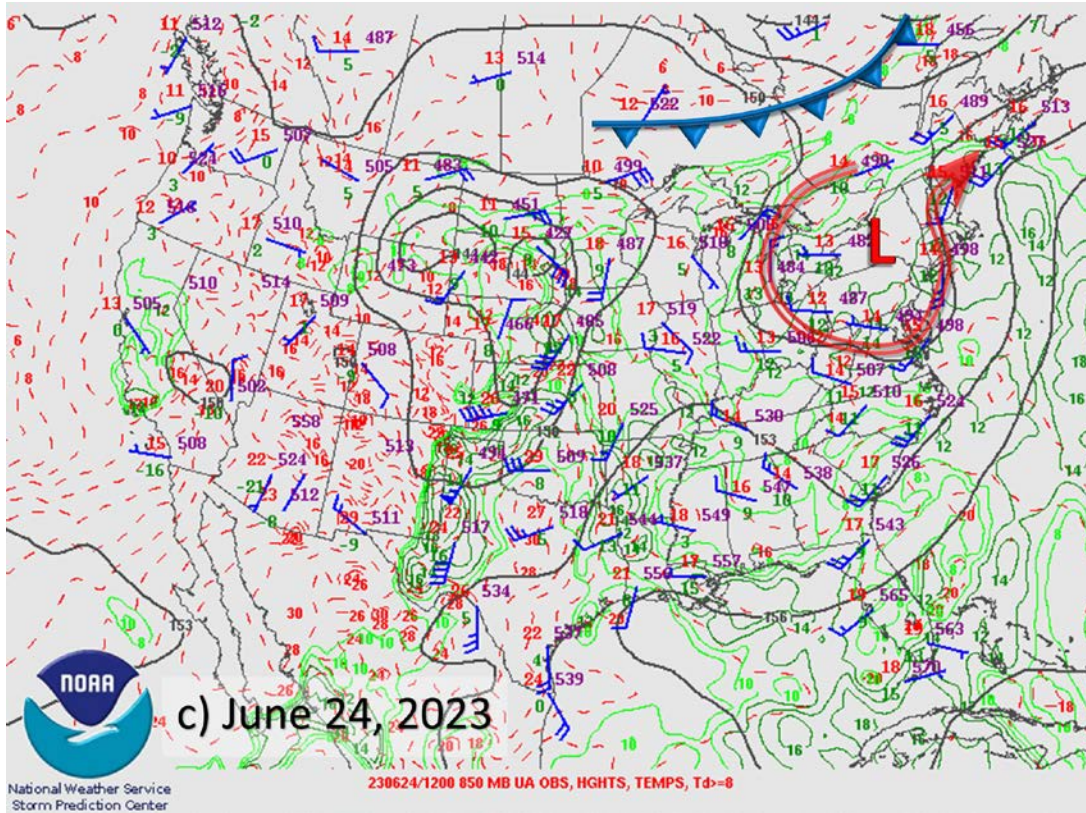
Figure 13: The 1200 UTC 850mb pattern for the CONUS on a) June 21, b) June 23, and c) June 24, 2023.
