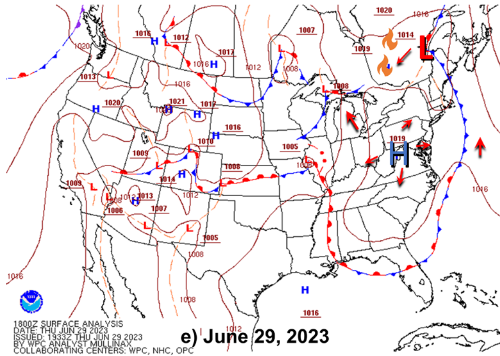
Figure 16: Surface analysis at 1800 UTC for a) June 25, b) June 26, c) June 27, d) June 28, e) June 29
