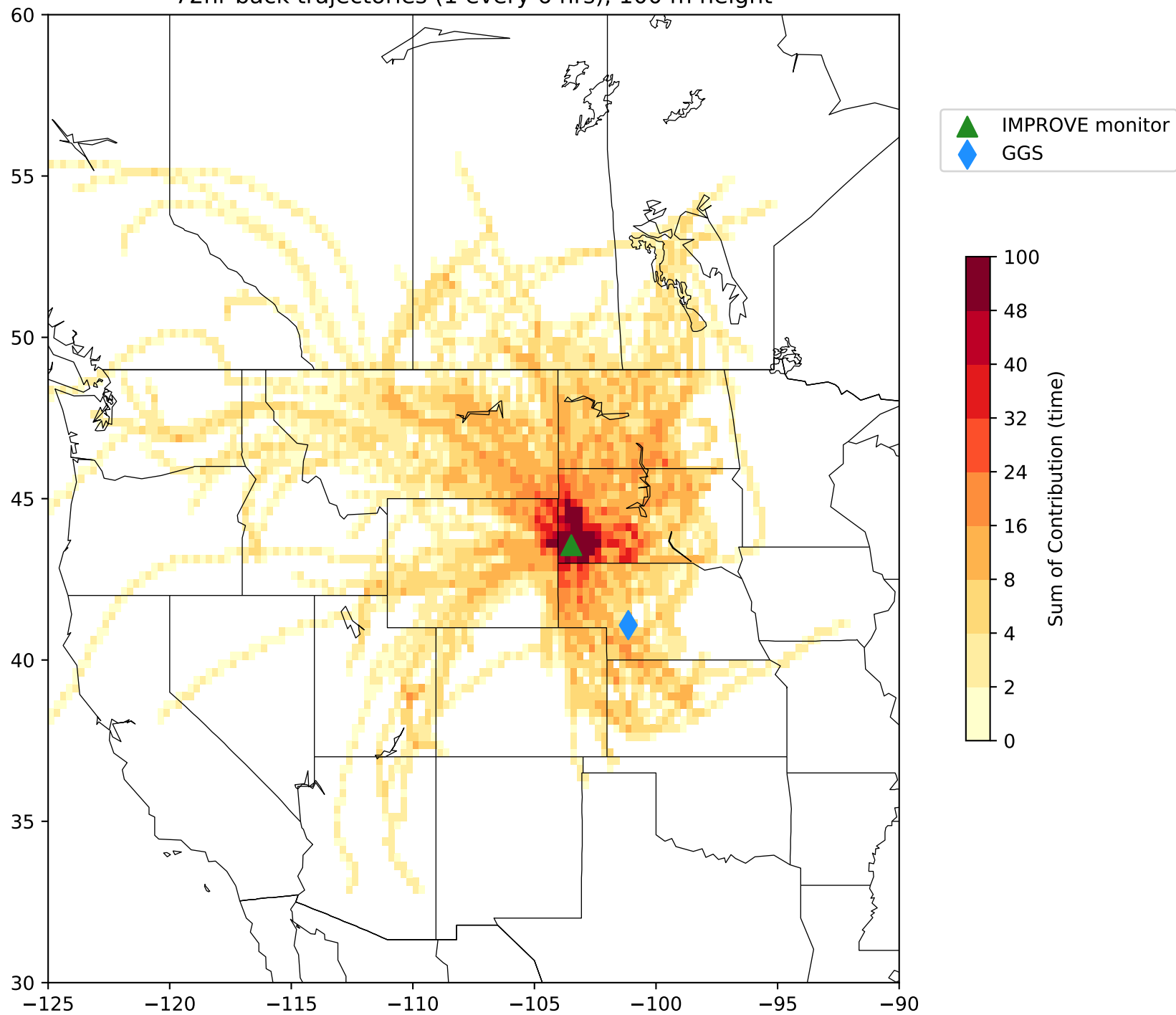
2009 Trajectory Time Plot for 20% Most Impaired Days at WICA1 72hr back trajectories (1 every 6 hrs), 100 m height
