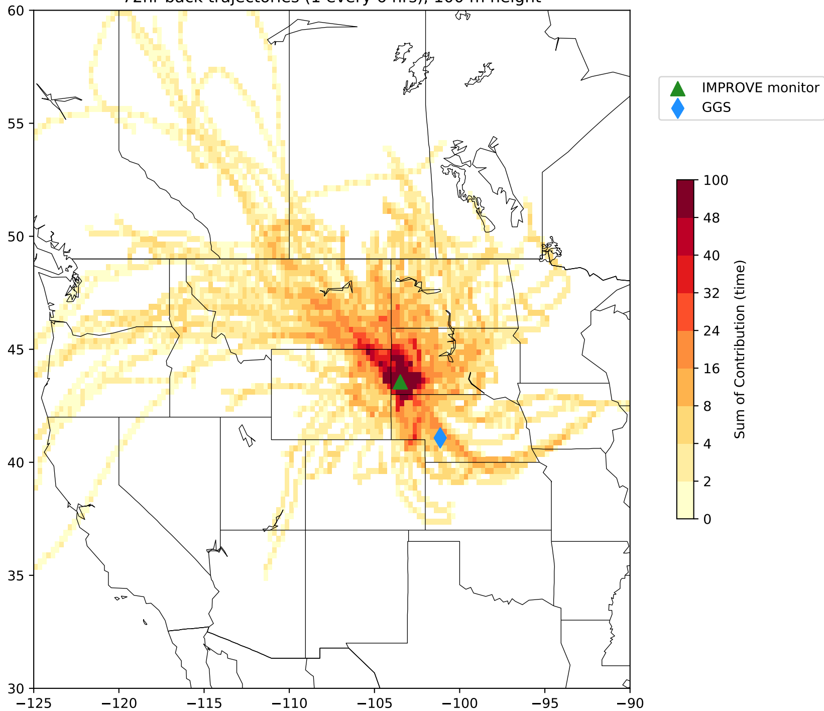
2015 Trajectory Time Plot for 20% Most Impaired Days at WICA1 72hr back trajectories (1 every 6 hrs), 100 m height
