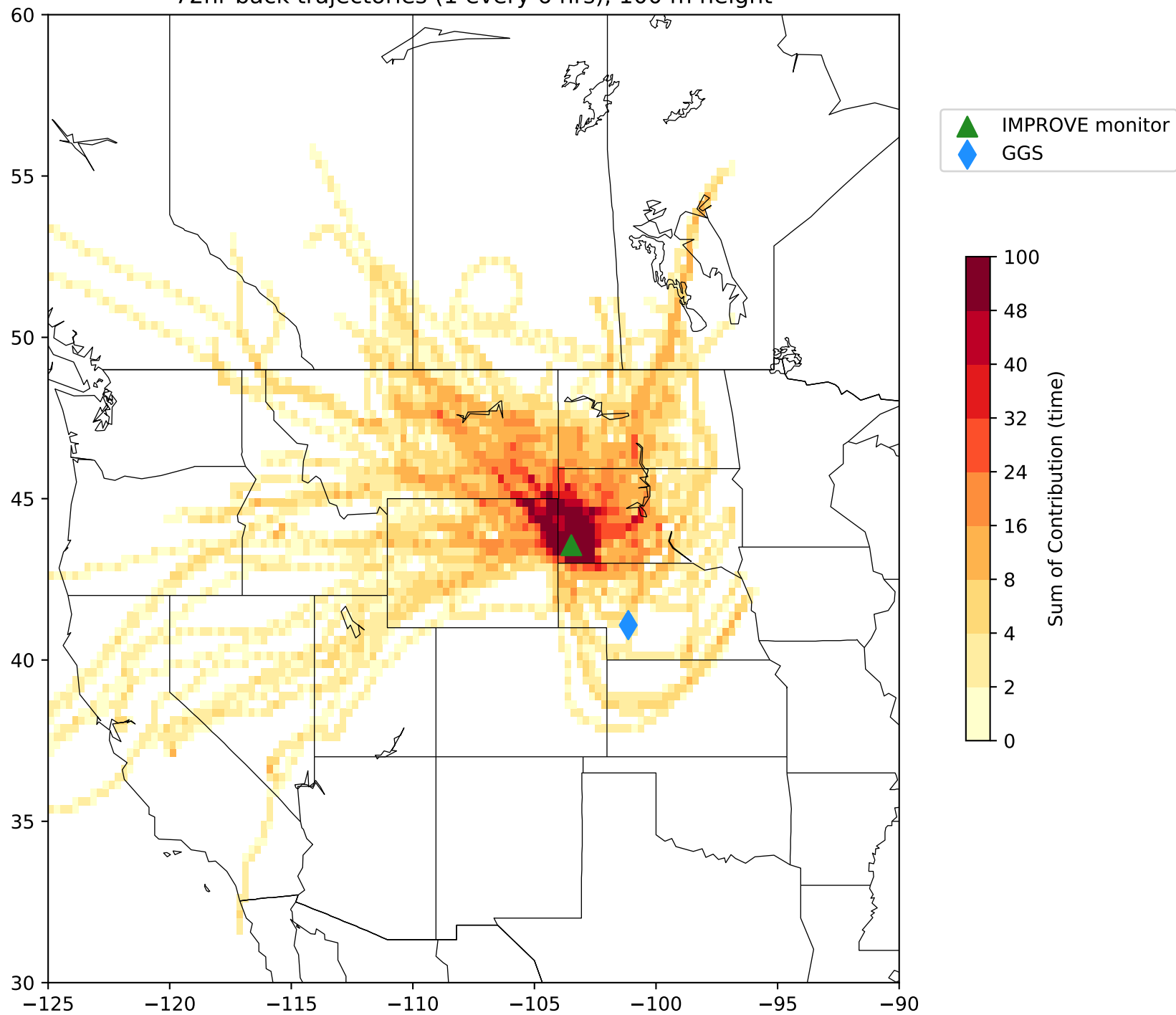
2017 Trajectory Time Plot for 20% Most Impaired Days at WICA1 72hr back trajectories (1 every 6 hrs), 100 m height
