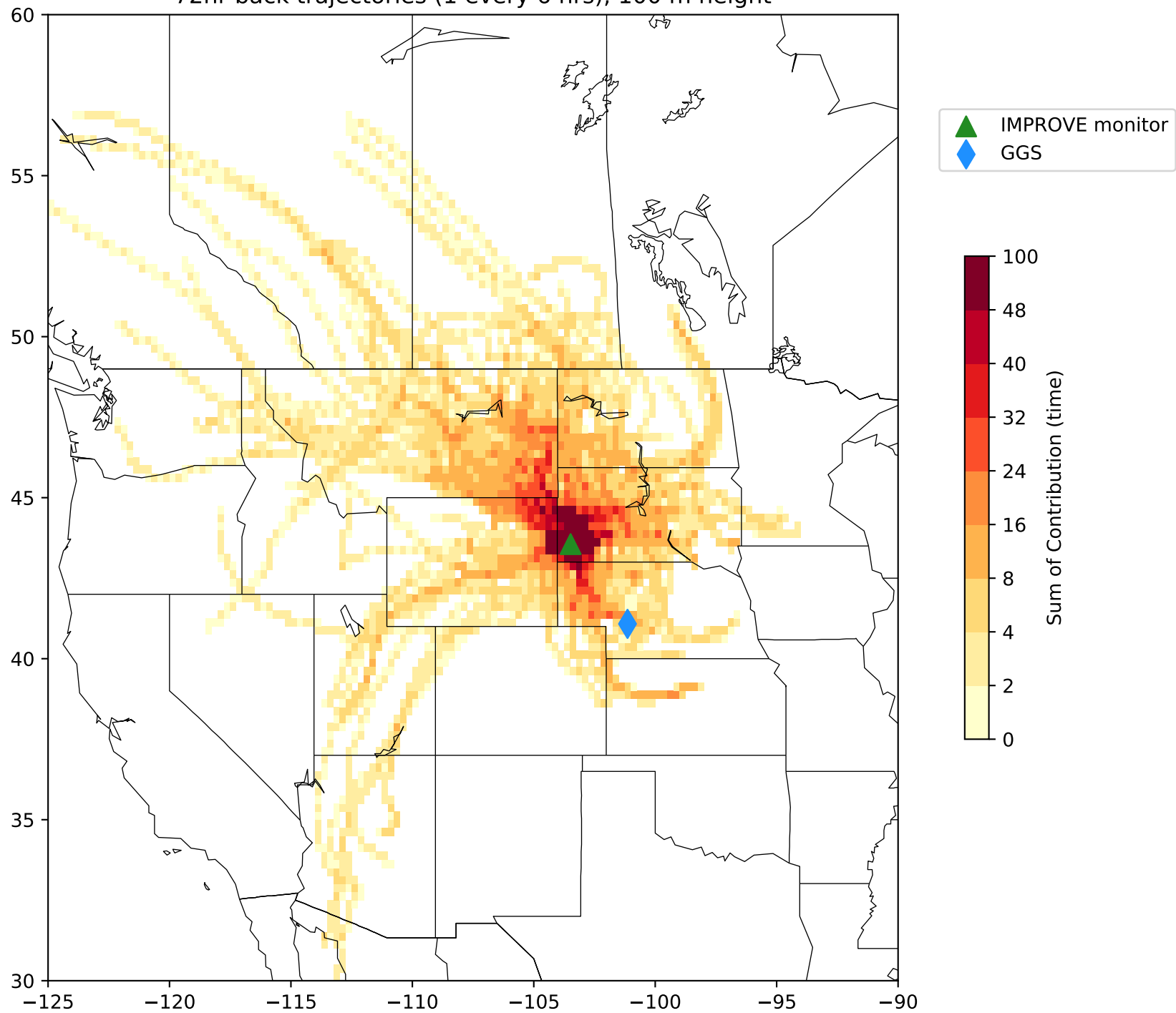
2021 Trajectory Time Plot for 20% Most Impaired Days at WICA1 72hr back trajectories (1 every 6 hrs), 100 m height
