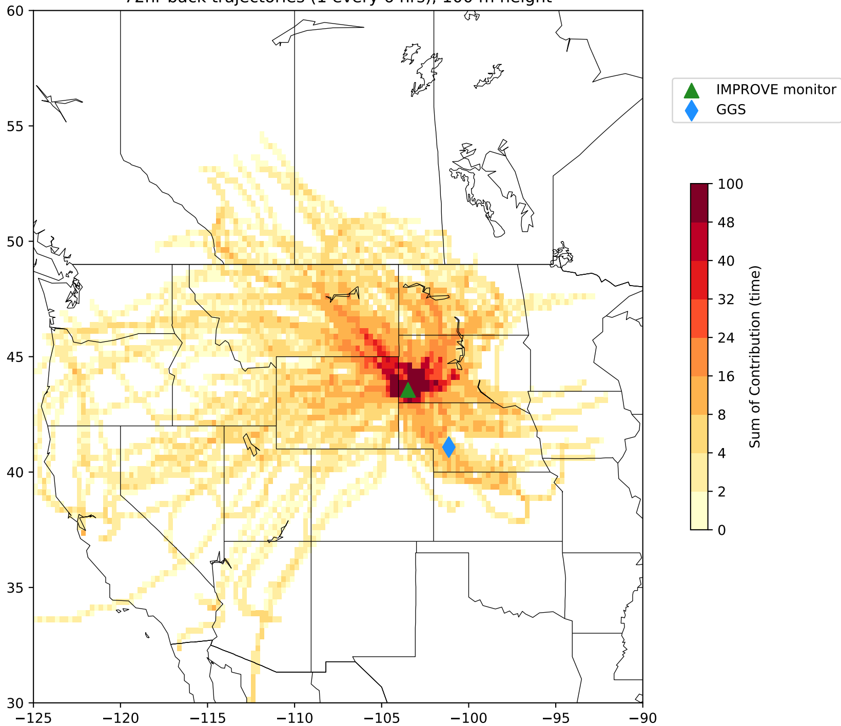
2011 Trajectory Time Plot for 20% Most Impaired Days at WICA1 72hr back trajectories (1 every 6 hrs), 100 m height
