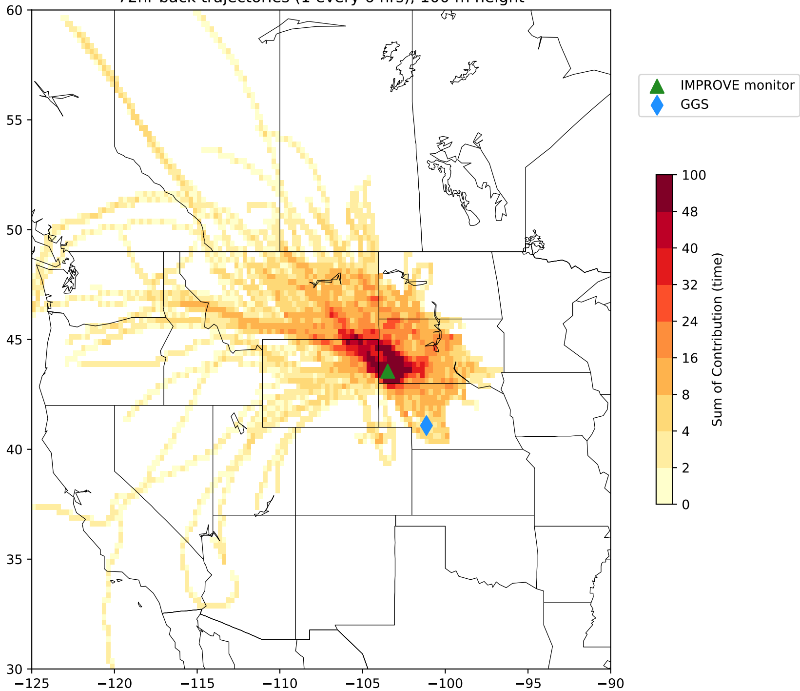
2019 Trajectory Time Plot for 20% Most Impaired Days at WICA1 72hr back trajectories (1 every 6 hrs), 100 m height
