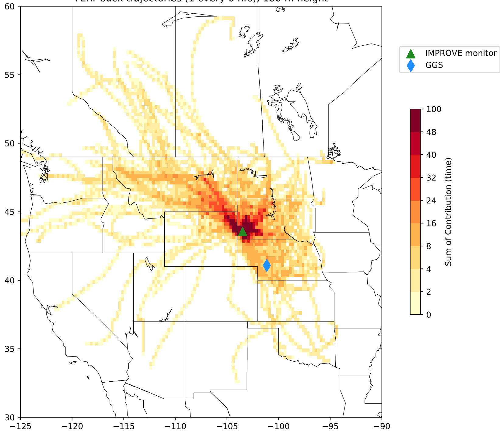
2013 Trajectory Time Plot for 20% Most Impaired Days at WICA1 72hr back trajectories (1 every 6 hrs), 100 m height
