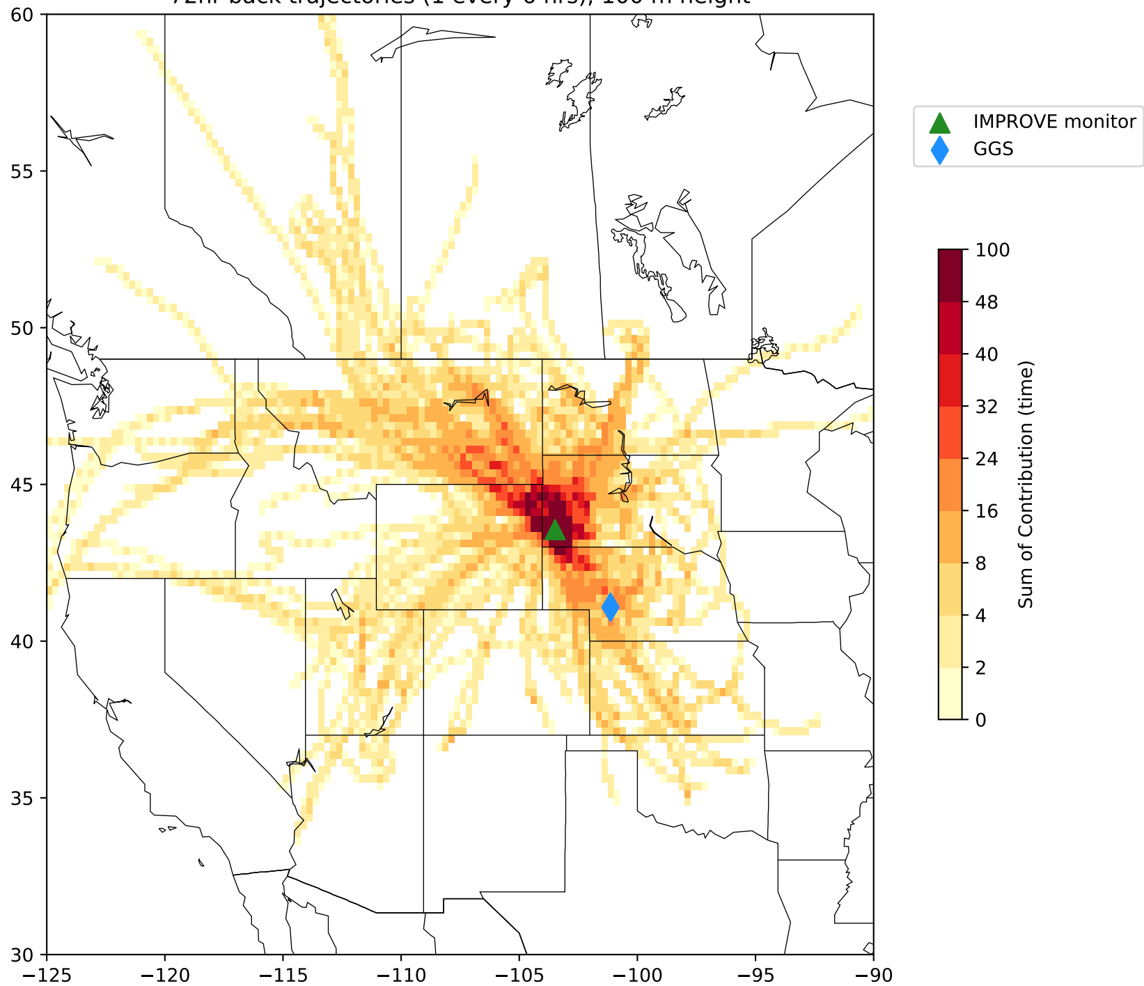
2016 Trajectory Time Plot for 20% Most Impaired Days at WICA1 72hr back trajectories (1 every 6 hrs), 100 m height
