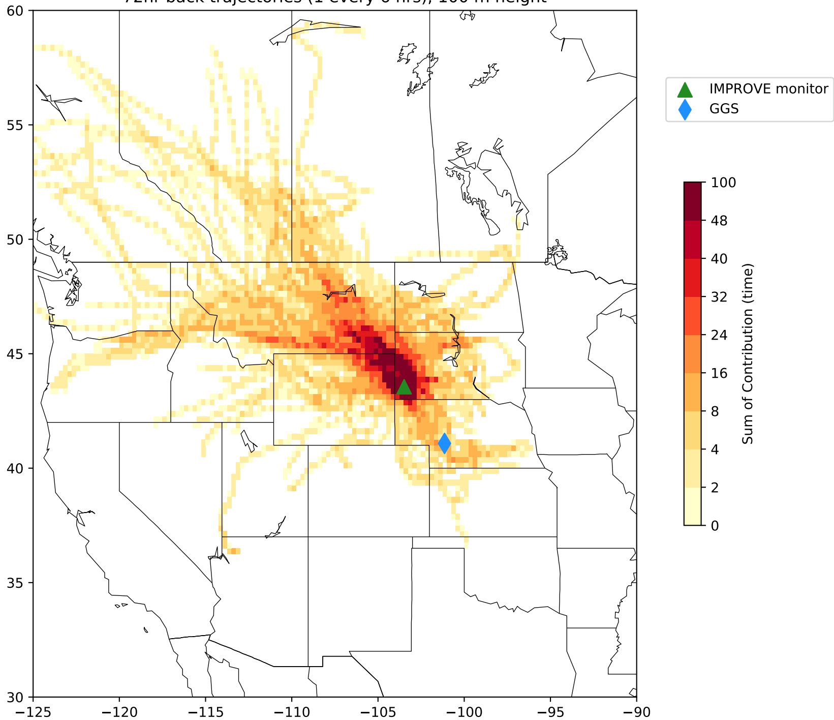
2020 Trajectory Time Plot for 20% Most Impaired Days at WICA1 72hr back trajectories (1 every 6 hrs), 100 m height
