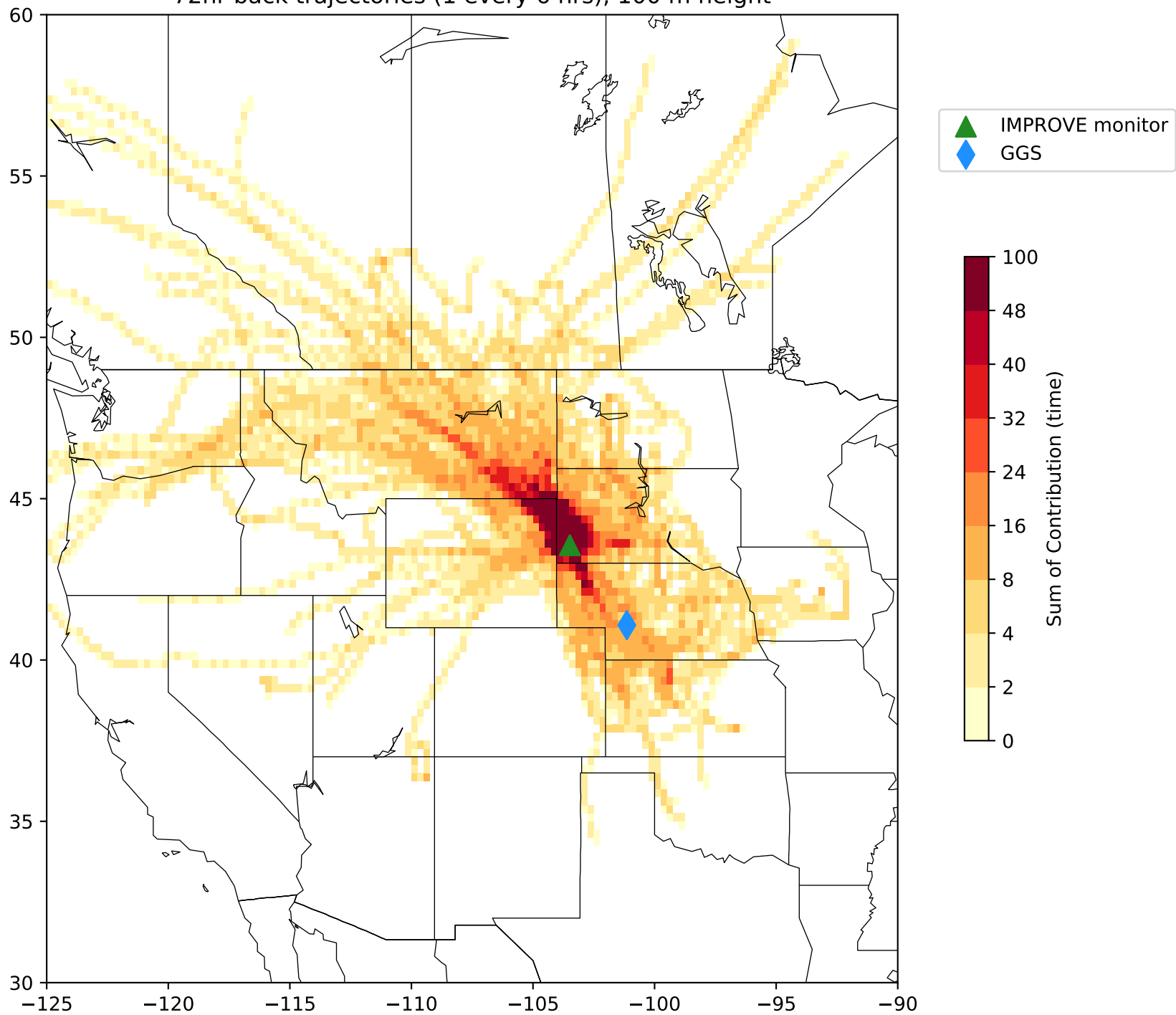
2008 Trajectory Time Plot for 20% Most Impaired Days at WICA1 72hr back trajectories (1 every 6 hrs), 100 m height
