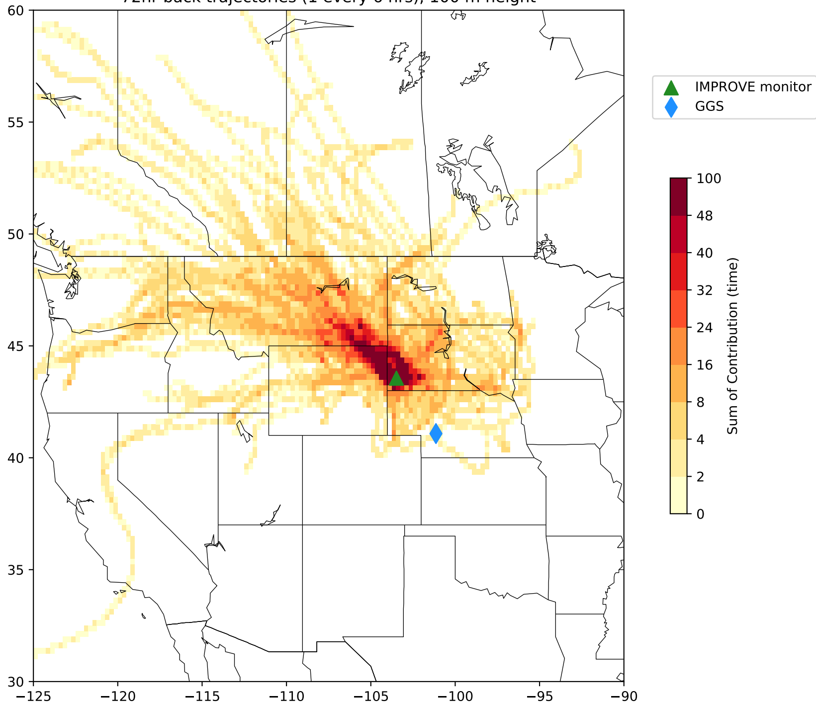
2014 Trajectory Time Plot for 20% Most Impaired Days at WICA1 72hr back trajectories (1 every 6 hrs), 100 m height
