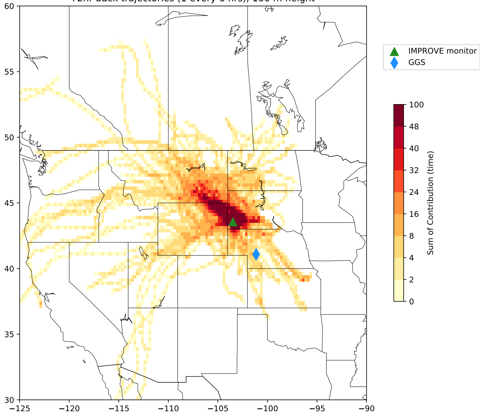
2010 Trajectory Time Plot for 20% Most Impaired Days at WICA1 72hr back trajectories (1 every 6 hrs), 100 m height
