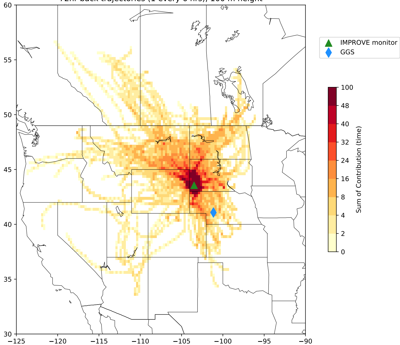
2018 Trajectory Time Plot for 20% Most Impaired Days at WICA1 72hr back trajectories (1 every 6 hrs), 100 m height
