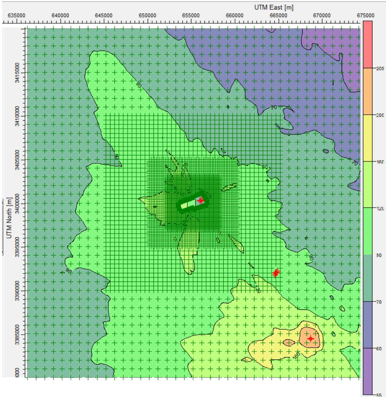
Figure 27: Predicted 99 th Percentile Daily Maximum 1-Hour SO 2 Concentrations Averaged Over 3 Years for the Area of Analysis for the Big Cajun II Due to All Sources
