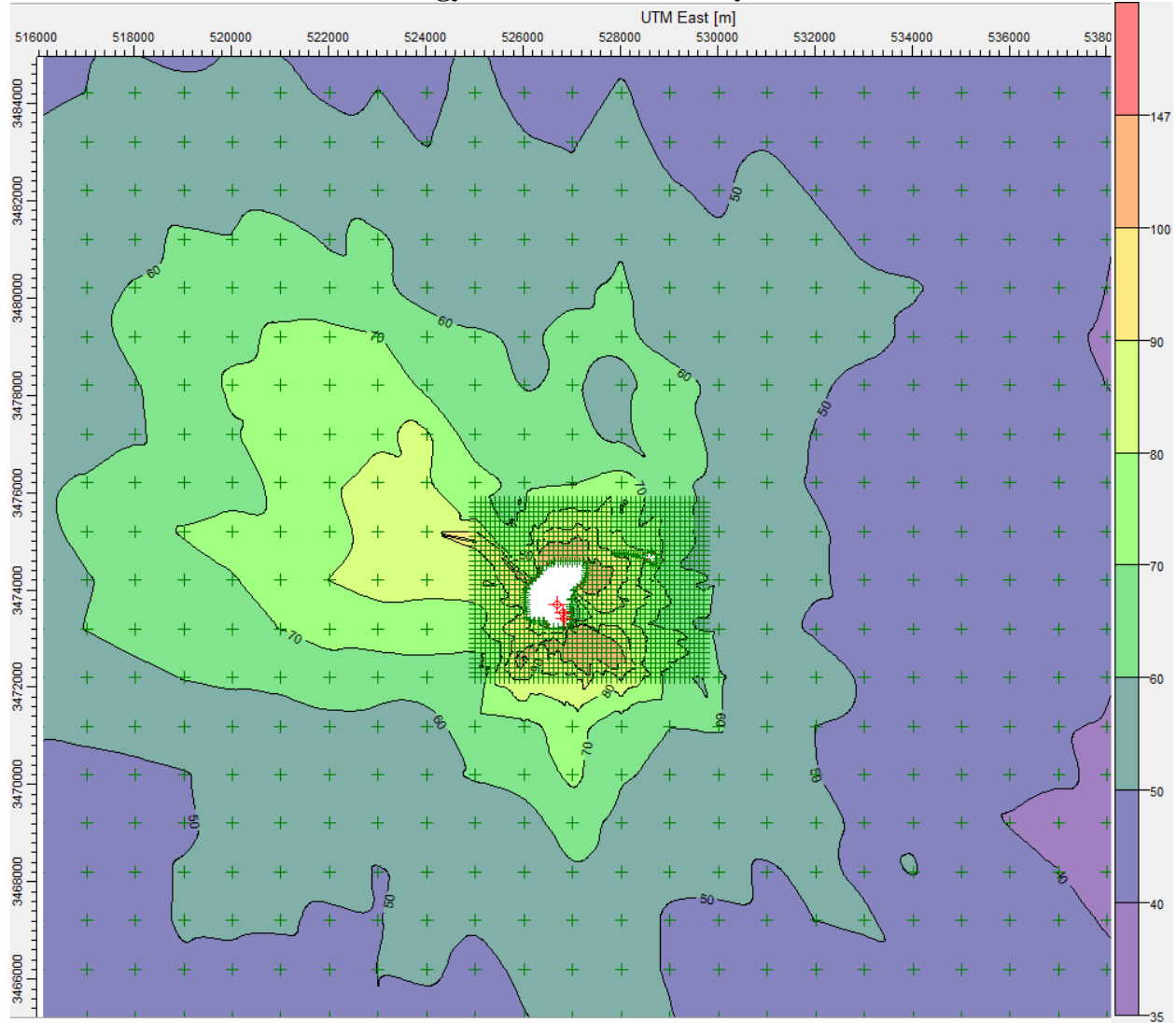
Figure 7: Predicted 99 th Percentile Daily Maximum 1-Hour SO 2 Concentrations Averaged Over 3 Years for the Brame Energy Center Area of Analysis
