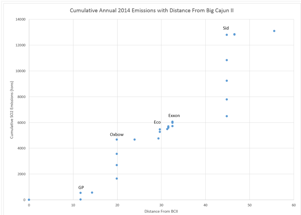
Figure 21: Cumulative 2014 Tons of SO 2 Emissions with Increasing Distance from Big Cajun II
