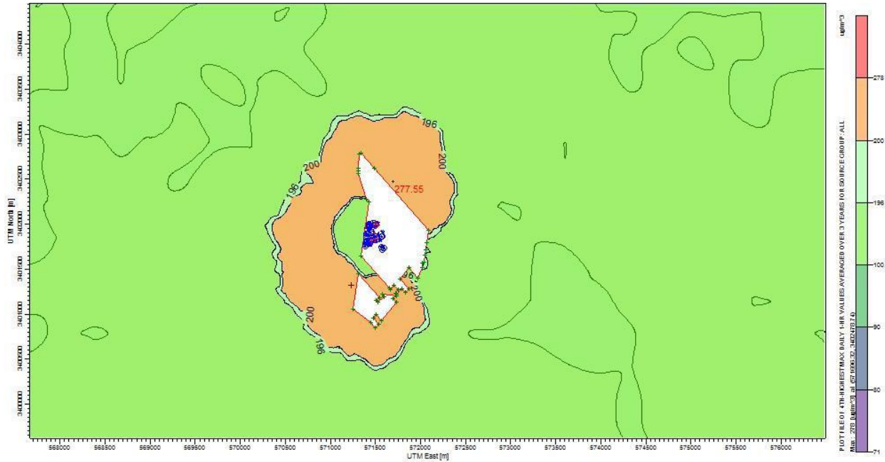
Figure 16: Near Field Impact Contour with Predicted 99 th Percentile Daily Maximum 1-Hour SO 2 Concentrations Averaged Over 3 Years for the Area of Analysis for the Evangeline Parish Area
