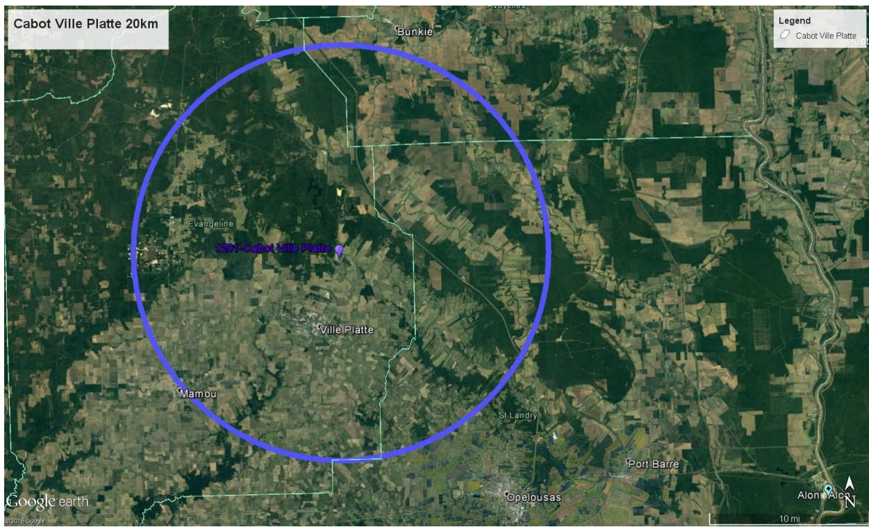
Figure 10: Area of Analysis for the Ville Platte Plant Area. The radius of the circle is 20 km.
