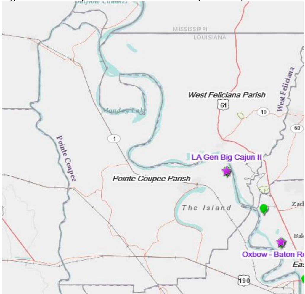
Figure 29: Boundary of the Intended Pointe Coupee Parish, Louisiana Unclassifiable Area
