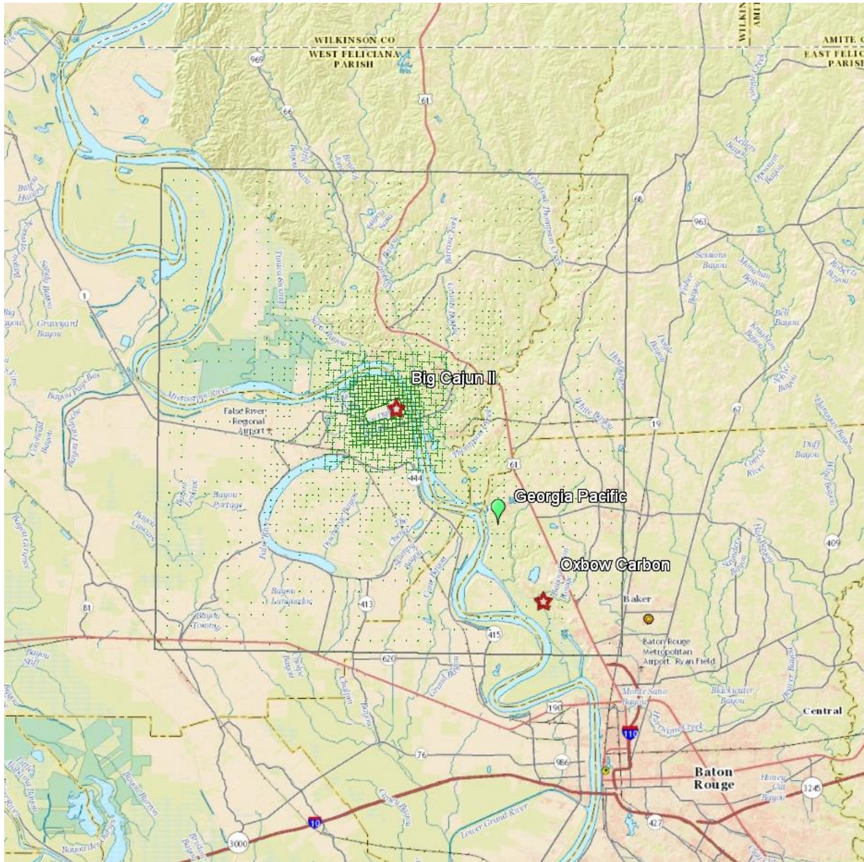
Figure 22: Area of Analysis for the Big Cajun II Area
