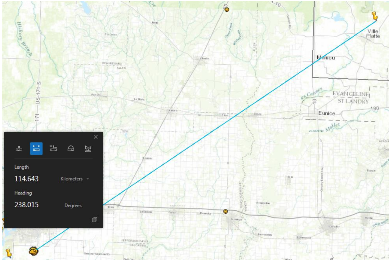
Figure 13: Area of Analysis and the NWS station in the Ville Platte Plant Area
