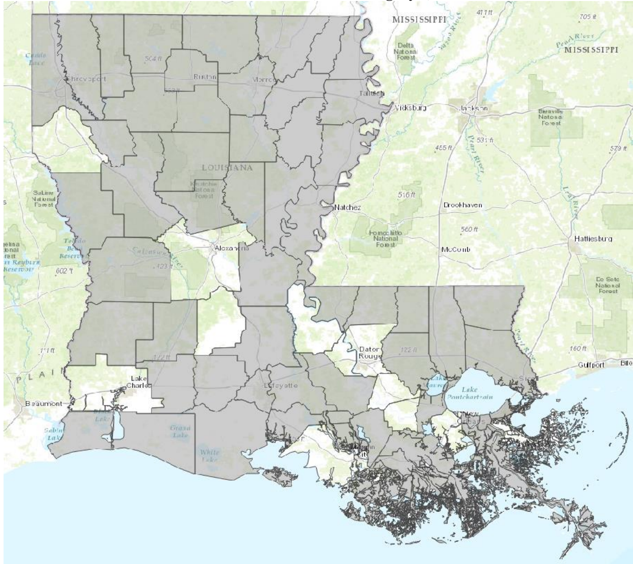
Figure 30: The EPA’s Intended Unclassifiable/Attainment Designations for Parishes in Louisiana Based on Absence of Information (shaded in gray) 19 .
