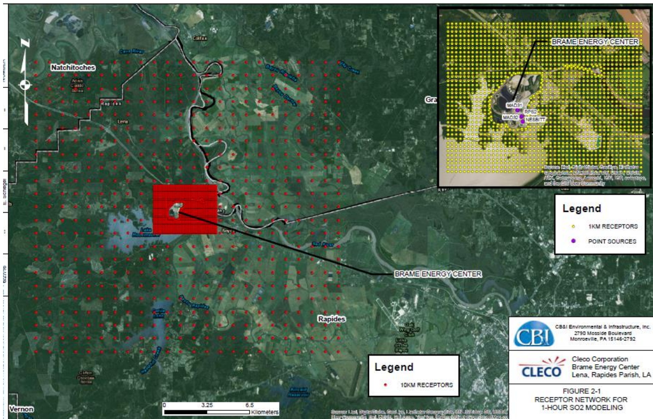
Figure 4: Receptor Grid for the Brame Energy Center Area
