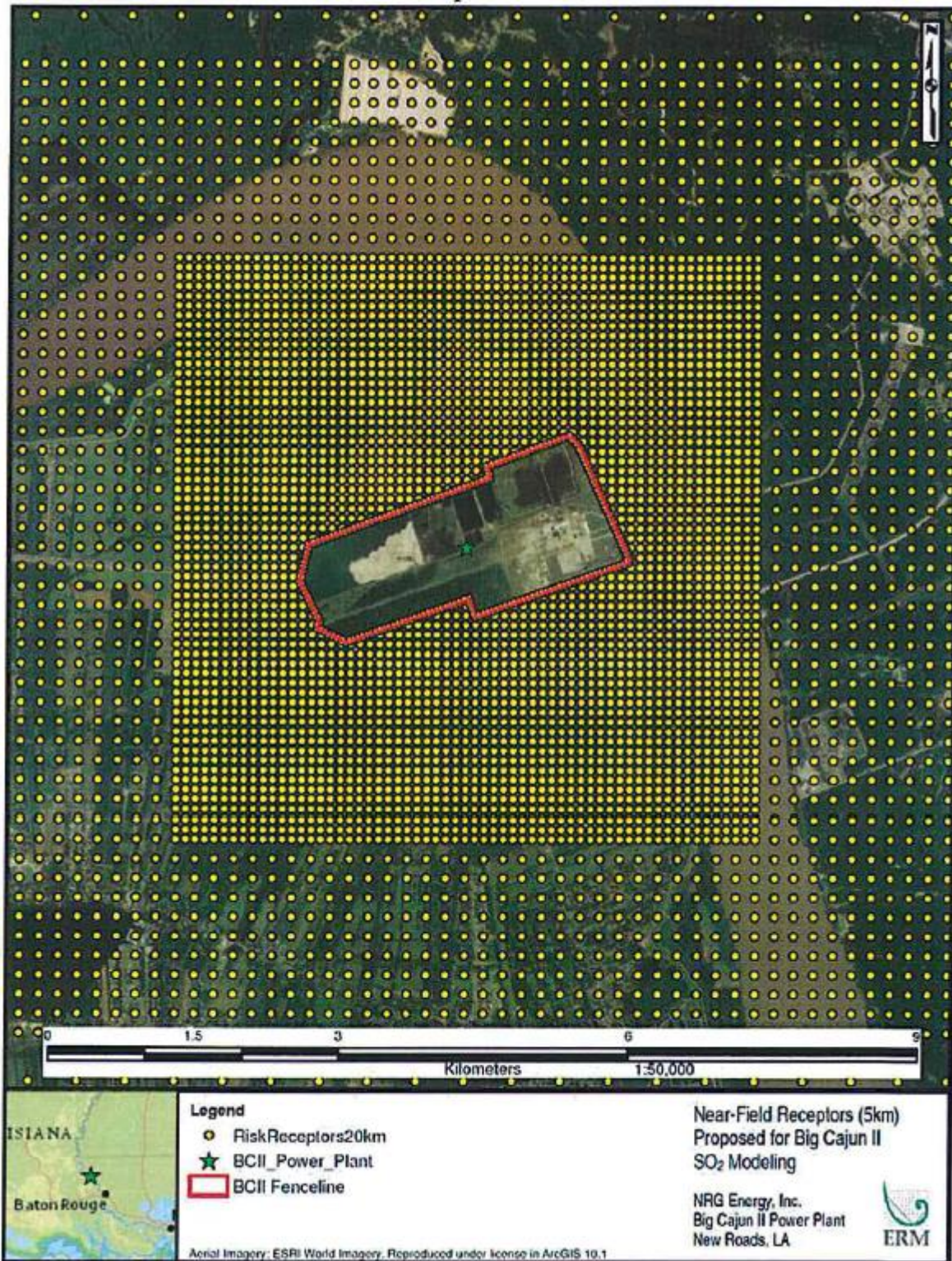
Figure 24. Near Field Receptor Grids for the Big Cajun II Area
