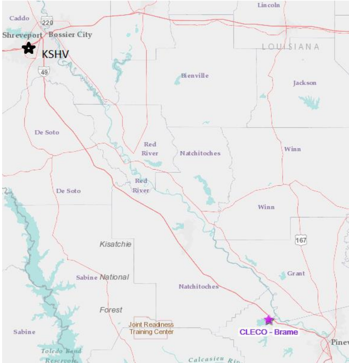
Figure 5: Brame Energy Center Area of Analysis and the Shreveport, Louisiana NWS station (KSHV)
