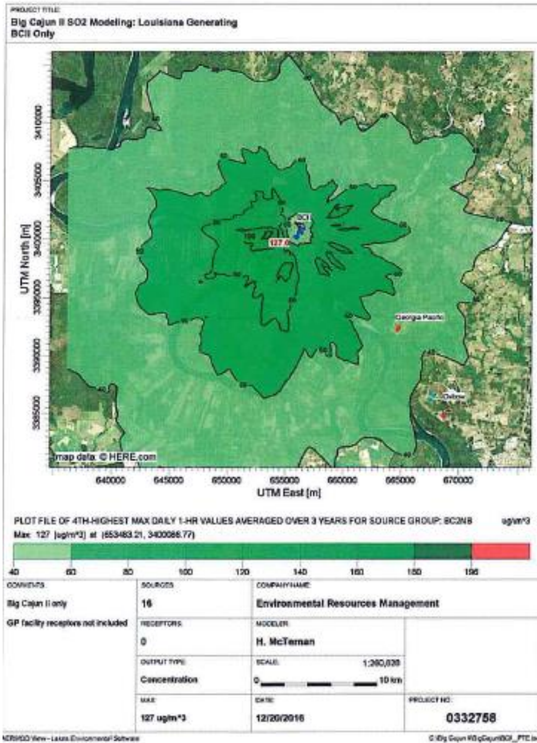
Figure 28: Predicted 99 th Percentile Daily Maximum 1-Hour SO 2 Concentrations Averaged Over 3 Years for the Area of Analysis for the Big Cajun II Area Due to Big Cajun II
