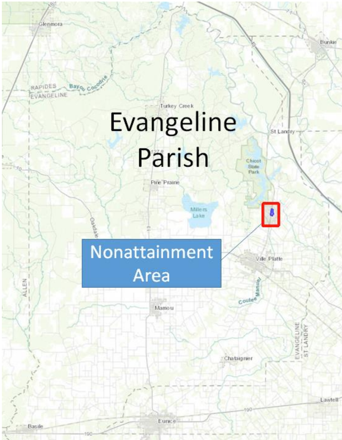
Figure 17: Intended Nonattainment Area for the SO 2 NAAQS for Evangeline Parish, Louisiana
