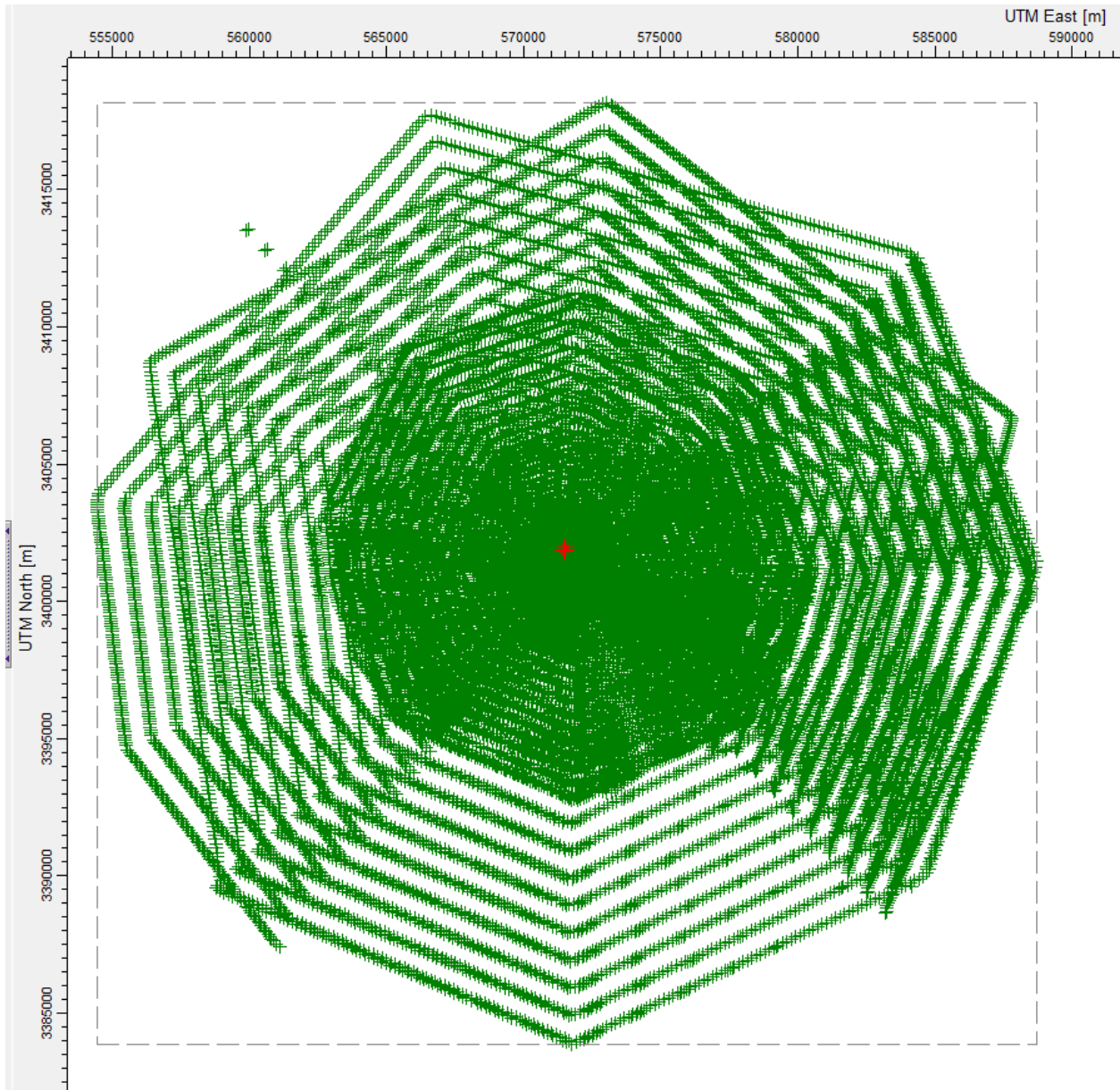
Figure 11: Far-Field Receptor Grid for the Ville Platte Plant Area
