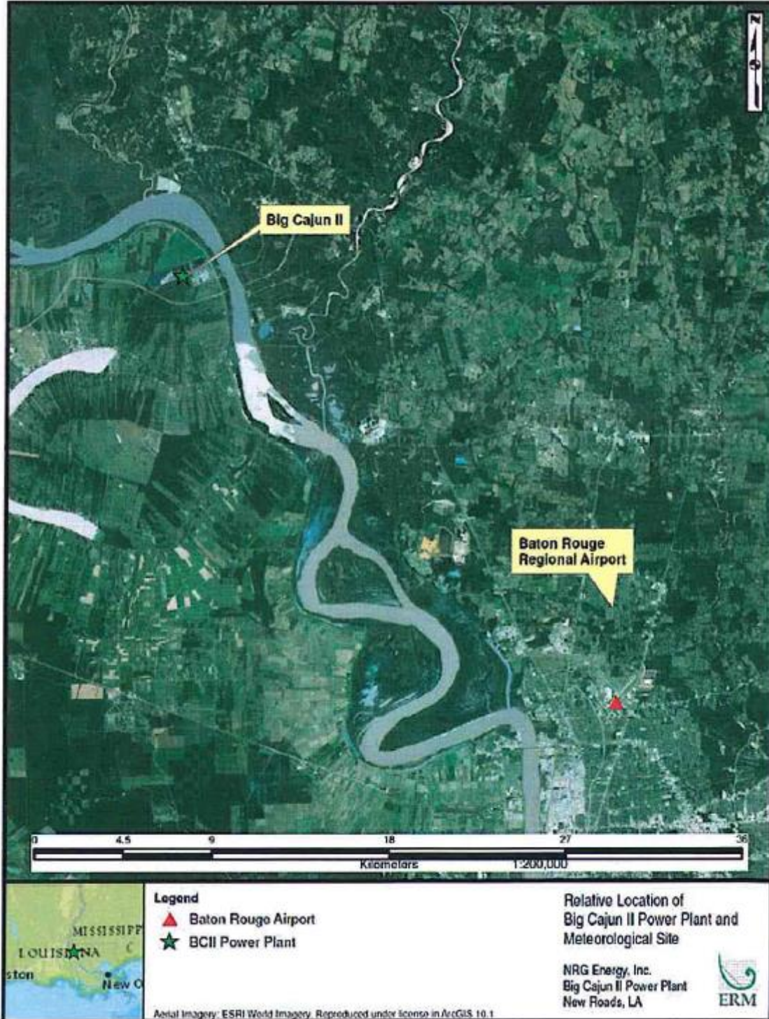
Figure 25: Area of Analysis and the NWS stations in the Big Cajun II Area
