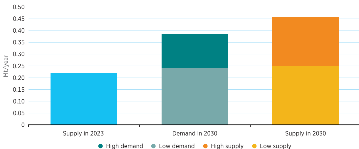
➤ FIGURE A1.7 Cobalt supply and demand in 2023 and 2030
