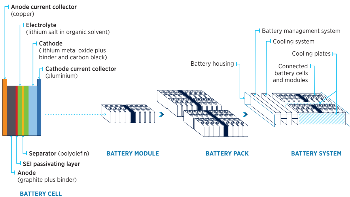
➤ FIGURE 6 Battery system components and internal components of a battery cell
