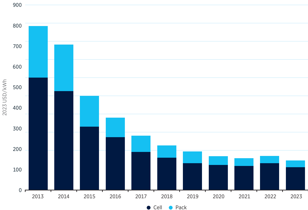
➤ FIGURE 3 Volume-weighted average price split for lithium-ion battery packs and cells, 2013-2023 (real USD 2023/kWh)
