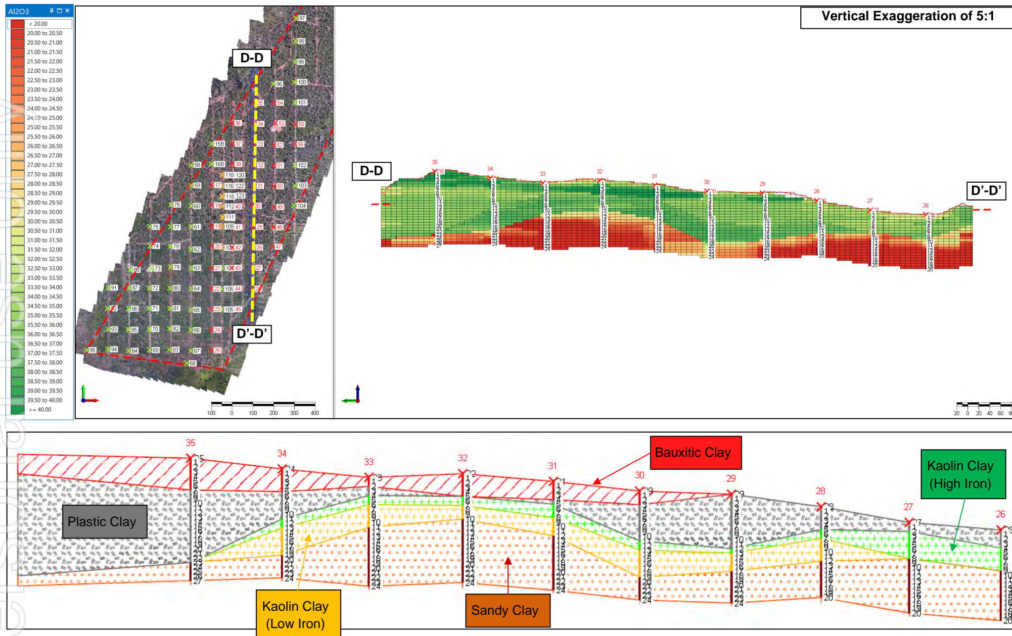
Figure IV. Section D-D to D'-D' (Long Section from North LHS of section to South RHS of section)
