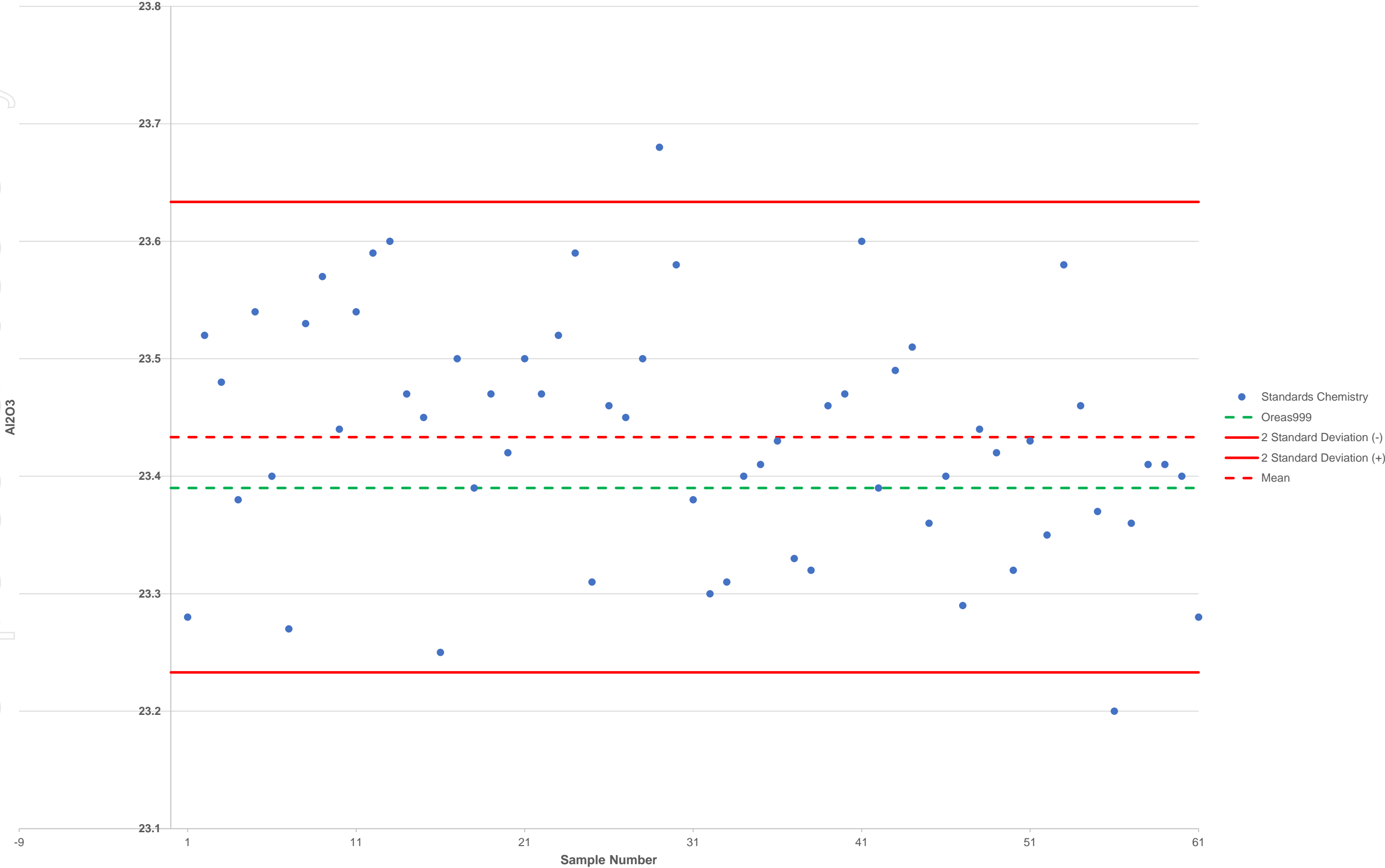
Control Charts for Phase II Standards - Al2O3
