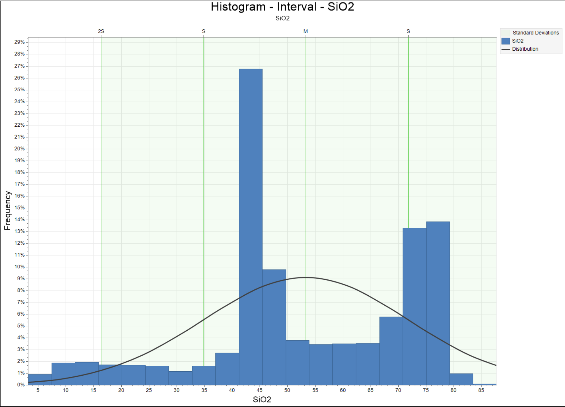
Figure 4.3 – SiO 2 Histogram
