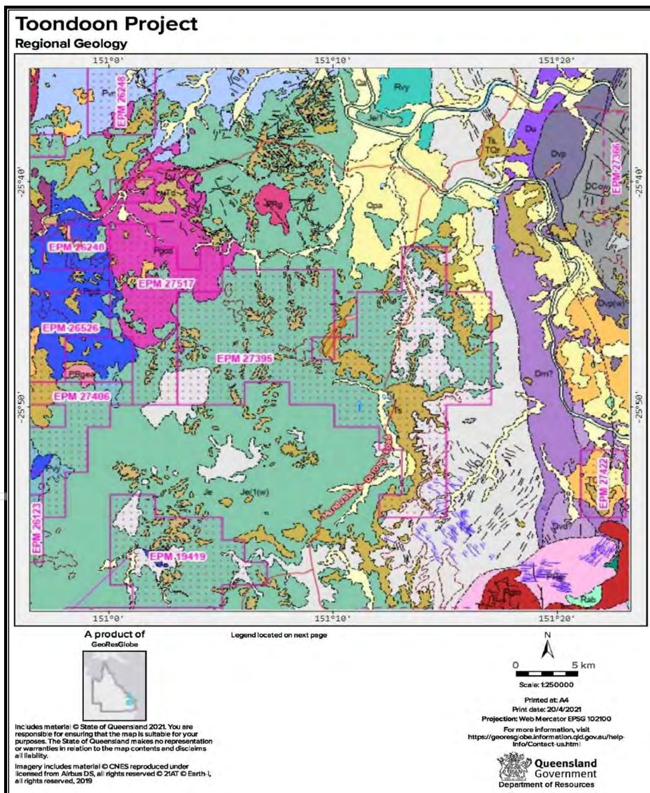
Figure 2.2 – Regional Geology
