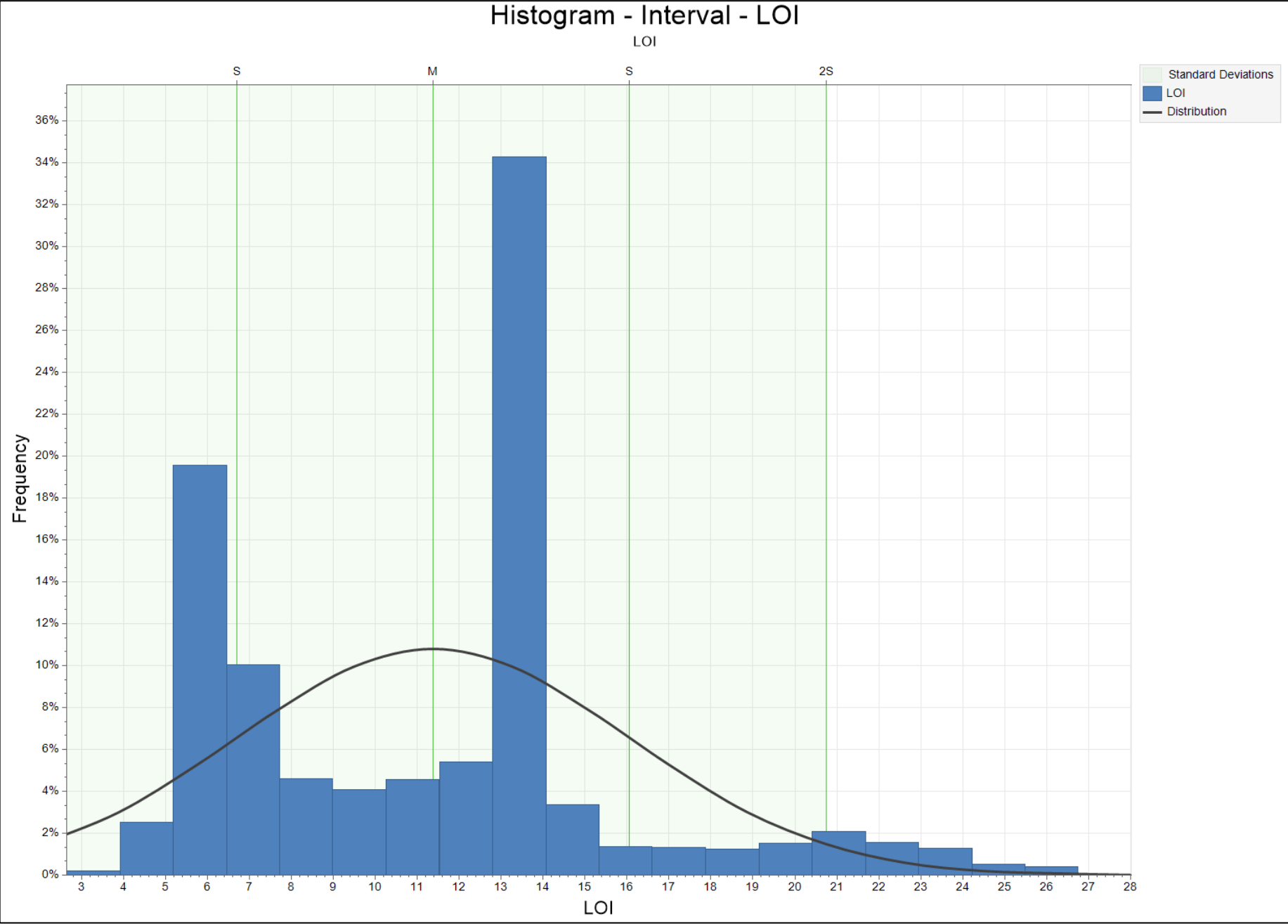
Figure 4.5 – LOI Histogram
