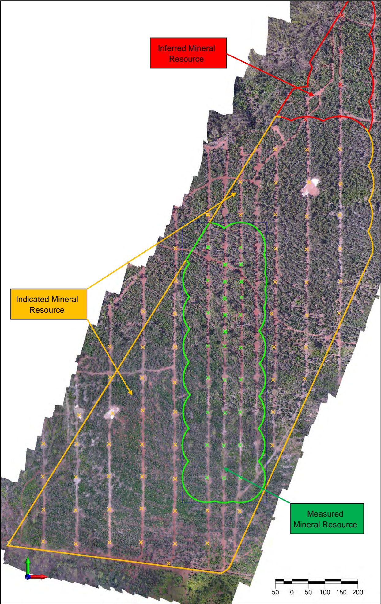
Figure 4.13 – Resource Classification
