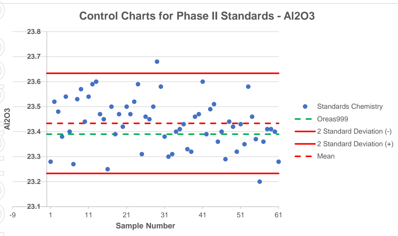
Figure 3.2 – QAQC of Phase II Standards – \text{Al}_2\text{O}_3
