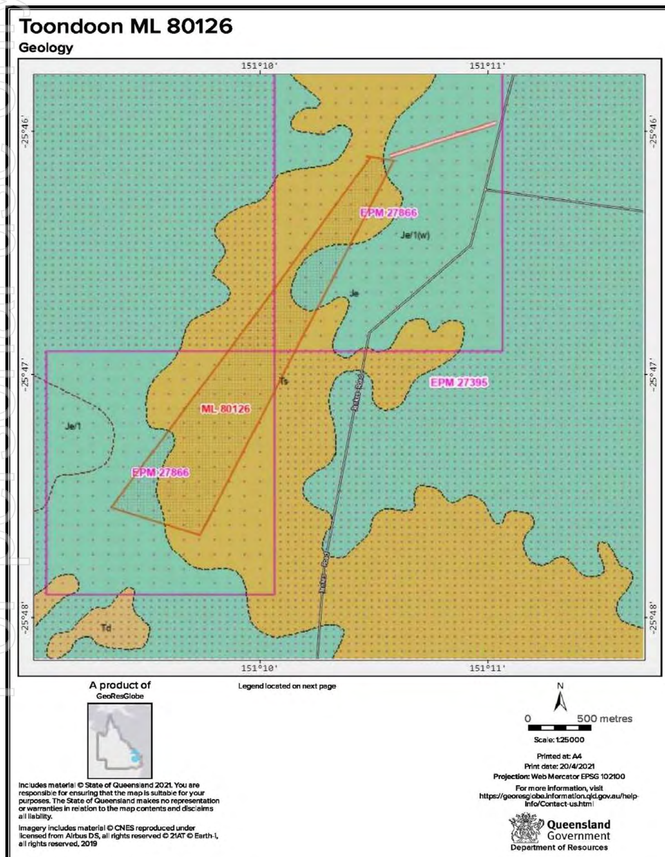
Figure 2.3 – Local Geology
