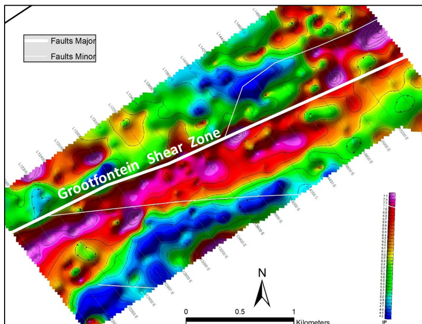
Figure 15: Result of the IP survey area at the Rothof Target: The Grootfontein Shear Zone is clearly marked
